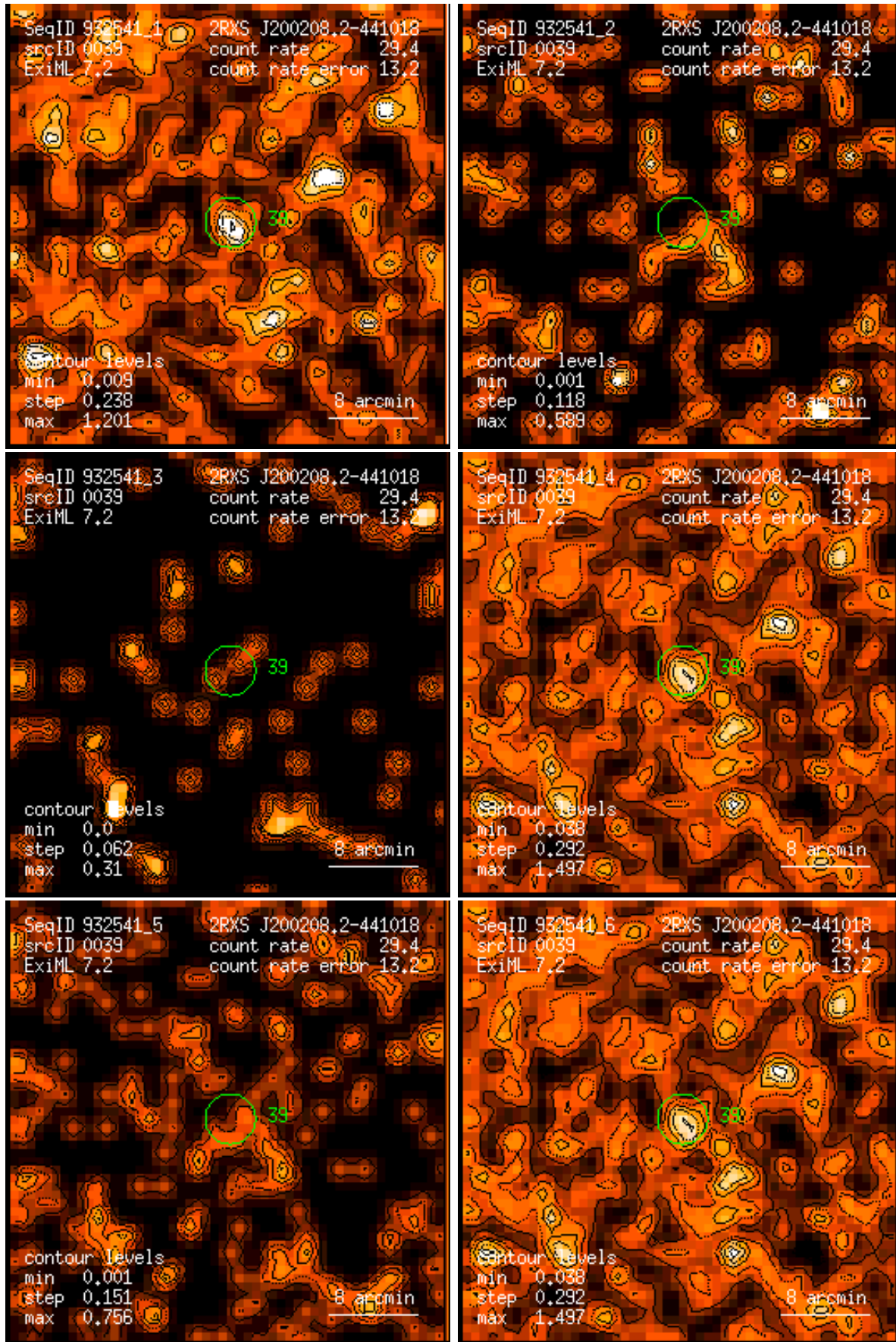
Figure 39: RASS 932541: detection 0039: band rate images, Gaussian filter: (1) PSPC channels 11 – 41, (2) 52 – 90, (3) 91 – 201, (4) 11 – 235, (5) 52 – 201, (6) 11 – 201. Broad band rates in counts/ks. Band rate contour levels in counts/ks/arcmin 2 .
