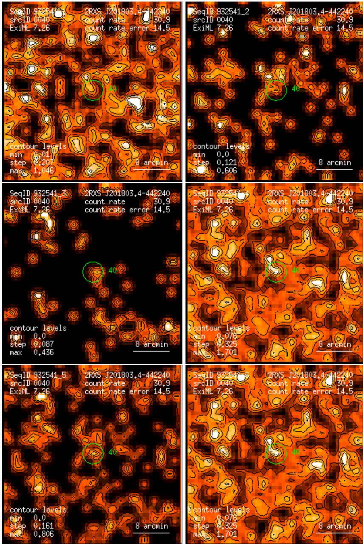
Figure 40: RASS 932541: detection 0040: band rate images, Gaussian filter: (1) PSPC channels 11 – 41, (2) 52 – 90, (3) 91 – 201, (4) 11 – 235, (5) 52 – 201, (6) 11 – 201. Broad band rates in counts/ks. Band rate contour levels in counts/ks/arcmin 2 .
