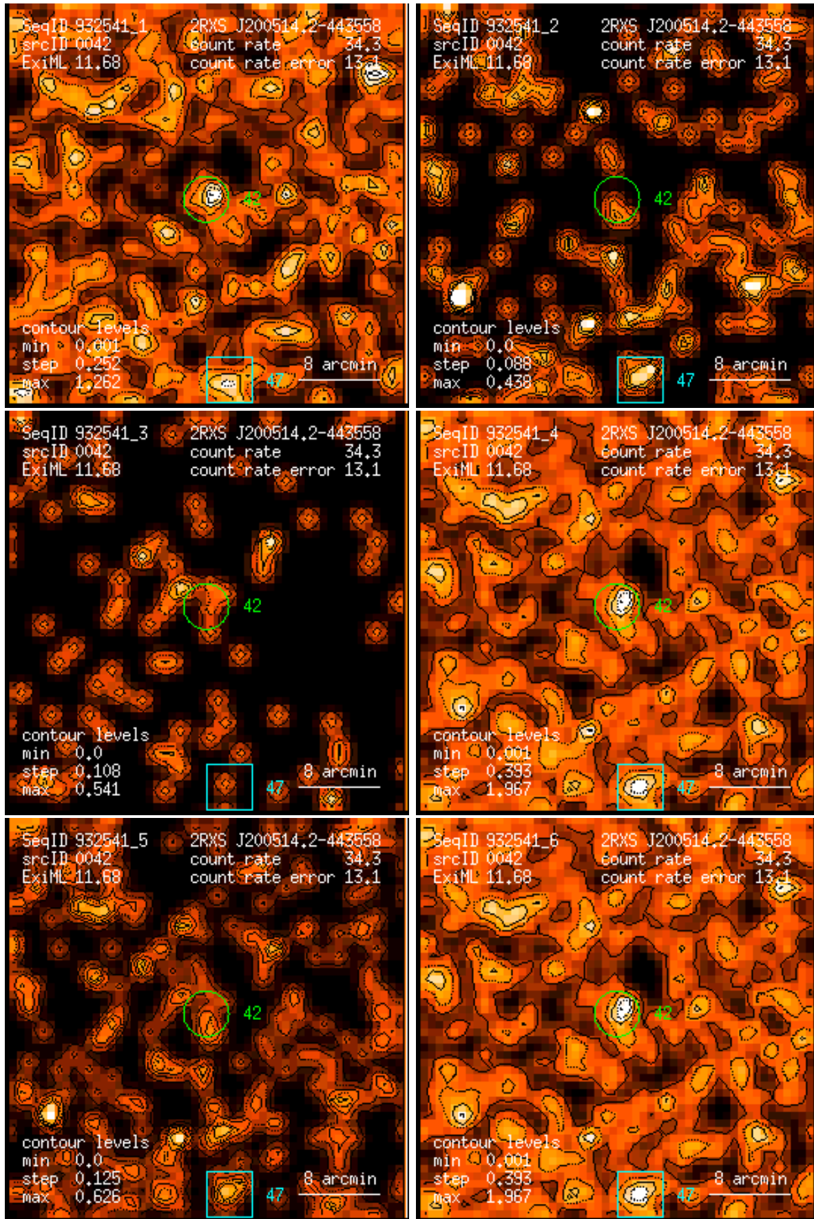
Figure 42: RASS 932541: detection 0042: band rate images, Gaussian filter: (1) PSPC channels 11 – 41, (2) 52 – 90, (3) 91 – 201, (4) 11 – 235, (5) 52 – 201, (6) 11 – 201. Broad band rates in counts/ks. Band rate contour levels in counts/ks/arcmin 2 .
