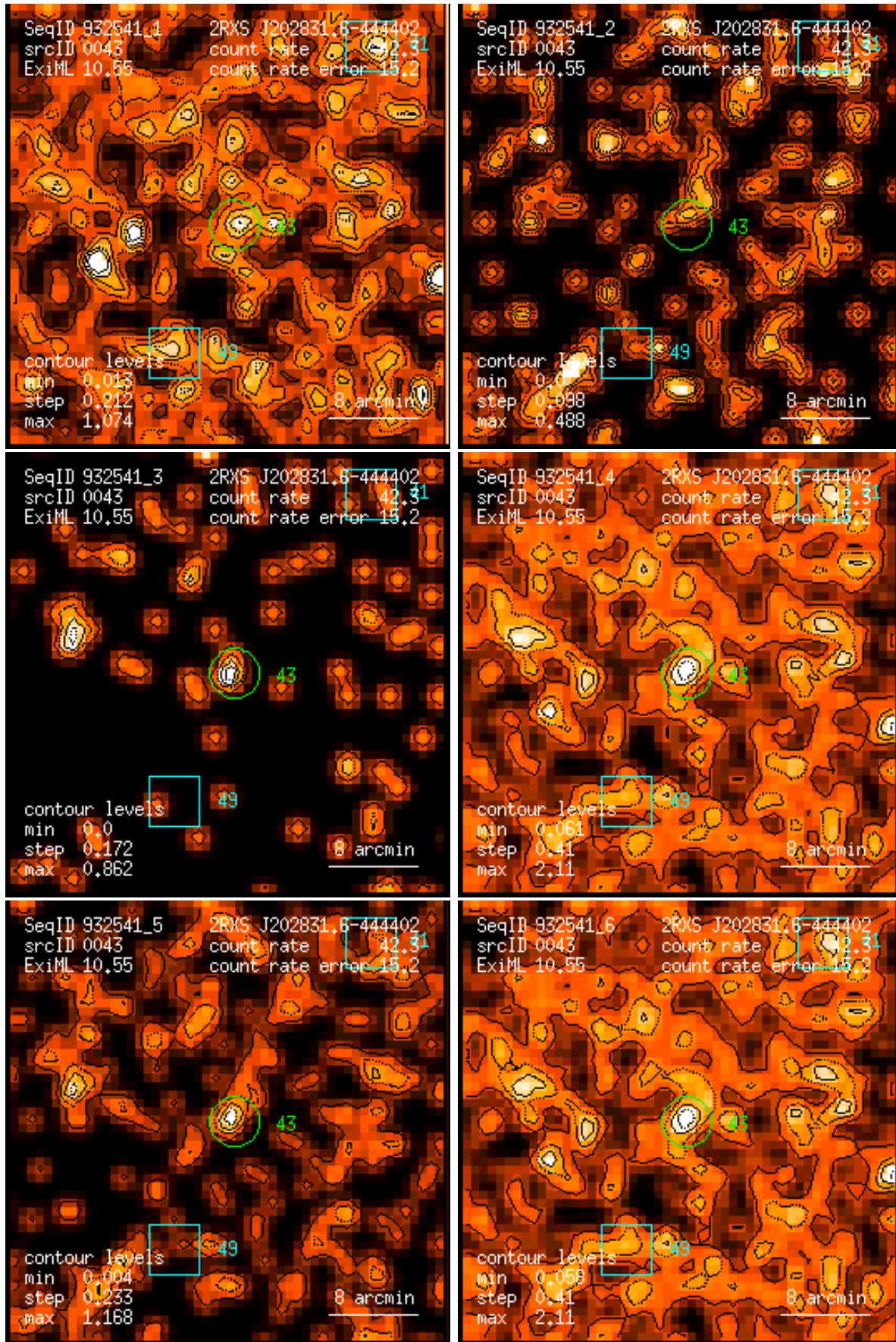
Figure 43: RASS 932541: detection 0043: band rate images, Gaussian filter: (1) PSPC channels 11 – 41, (2) 52 – 90, (3) 91 – 201, (4) 11 – 235, (5) 52 – 201, (6) 11 – 201. Broad band rates in counts/ks. Band rate contour levels in counts/ks/arcmin 2 .
