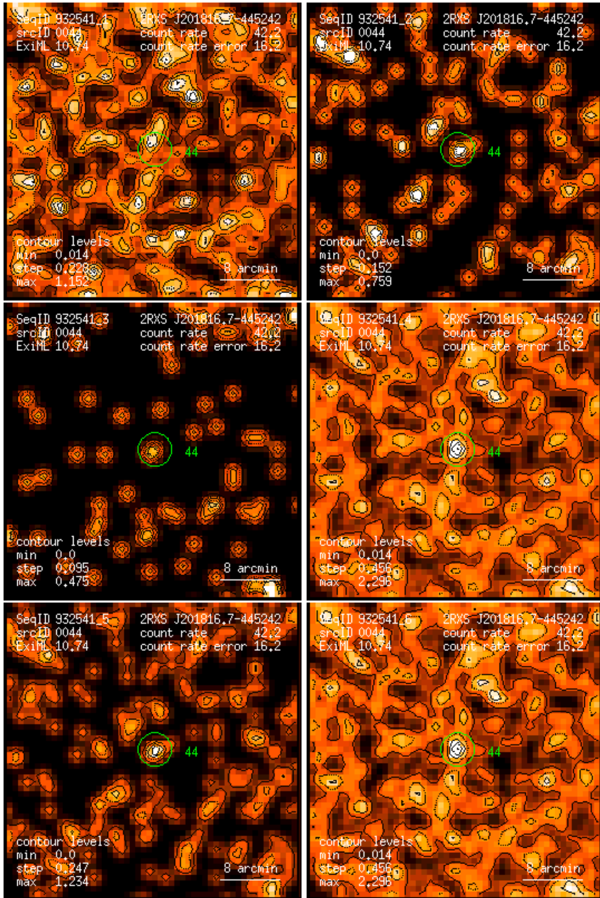
Figure 44: RASS 932541: detection 0044: band rate images, Gaussian filter: (1) PSPC channels 11 – 41, (2) 52 – 90, (3) 91 – 201, (4) 11 – 235, (5) 52 – 201, (6) 11 – 201. Broad band rates in counts/ks. Band rate contour levels in counts/ks/arcmin 2 .
