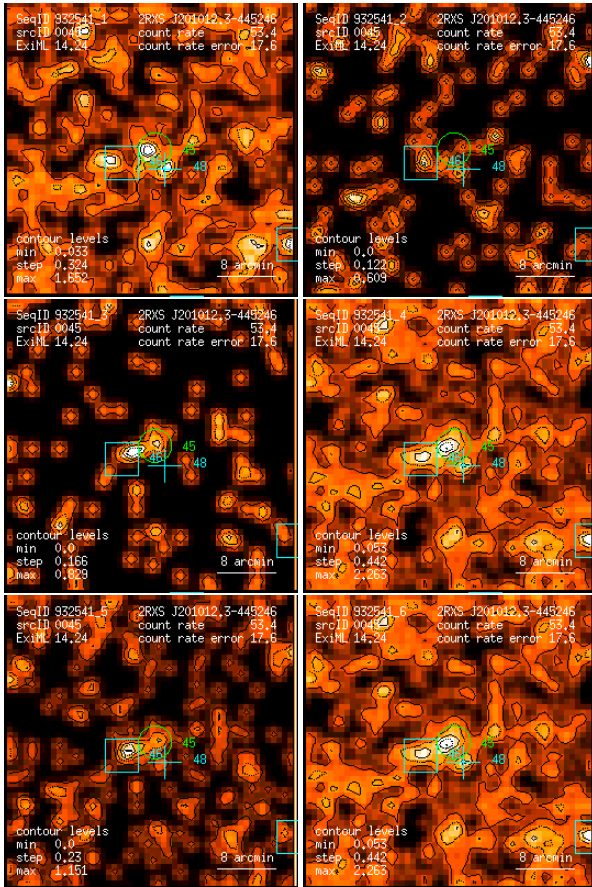
Figure 45: RASS 932541: detection 0045: band rate images, Gaussian filter: (1) PSPC channels 11 – 41, (2) 52 – 90, (3) 91 – 201, (4) 11 – 235, (5) 52 – 201, (6) 11 – 201. Broad band rates in counts/ks. Band rate contour levels in counts/ks/arcmin 2 .
