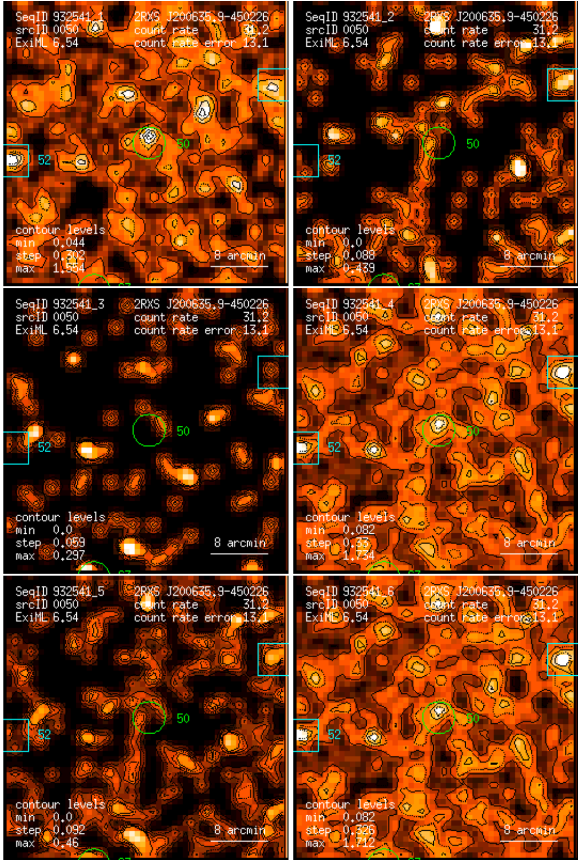
Figure 50: RASS 932541: detection 0050: band rate images, Gaussian filter: (1) PSPC channels 11 – 41, (2) 52 – 90, (3) 91 – 201, (4) 11 – 235, (5) 52 – 201, (6) 11 – 201. Broad band rates in counts/ks. Band rate contour levels in counts/ks/arcmin 2 .
