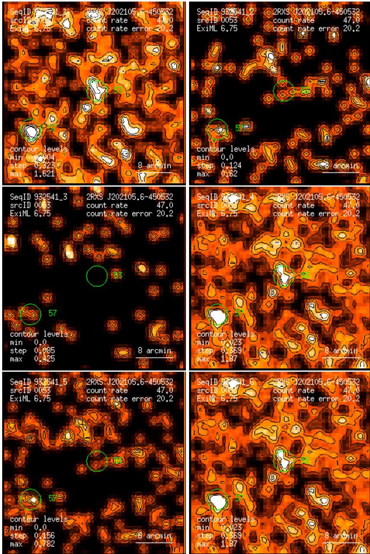
Figure 53: RASS 932541: detection 0053: band rate images, Gaussian filter: (1) PSPC channels 11 – 41, (2) 52 – 90, (3) 91 – 201, (4) 11 – 235, (5) 52 – 201, (6) 11 – 201. Broad band rates in counts/ks. Band rate contour levels in counts/ks/arcmin 2 .
