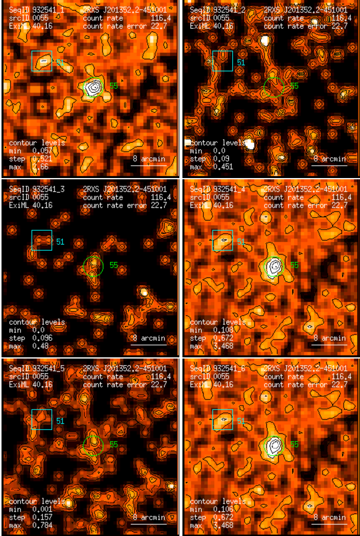
Figure 55: RASS 932541: detection 0055: band rate images, Gaussian filter: (1) PSPC channels 11 – 41, (2) 52 – 90, (3) 91 – 201, (4) 11 – 235, (5) 52 – 201, (6) 11 – 201. Broad band rates in counts/ks. Band rate contour levels in counts/ks/arcmin 2 .
