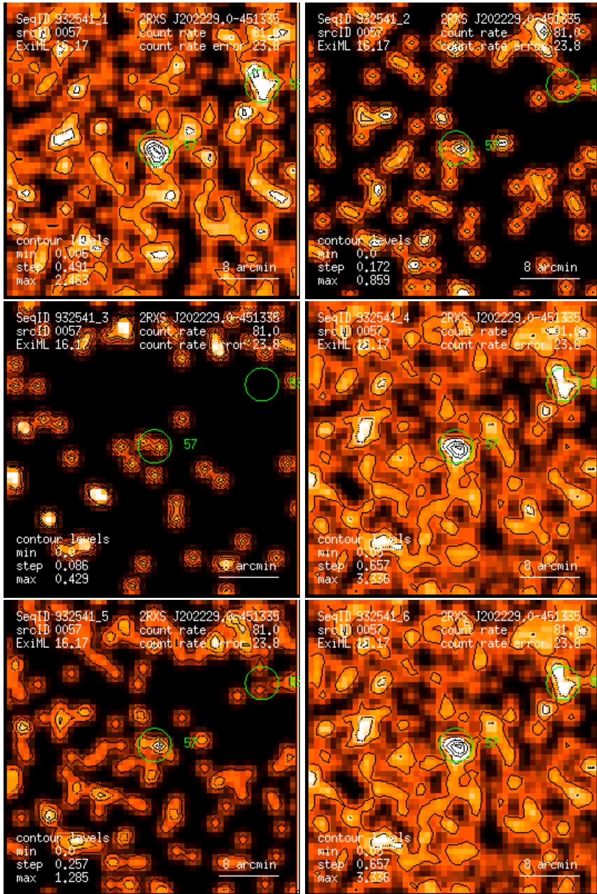
Figure 57: RASS 932541: detection 0057: band rate images, Gaussian filter: (1) PSPC channels 11 – 41, (2) 52 – 90, (3) 91 – 201, (4) 11 – 235, (5) 52 – 201, (6) 11 – 201. Broad band rates in counts/ks. Band rate contour levels in counts/ks/arcmin 2 .
