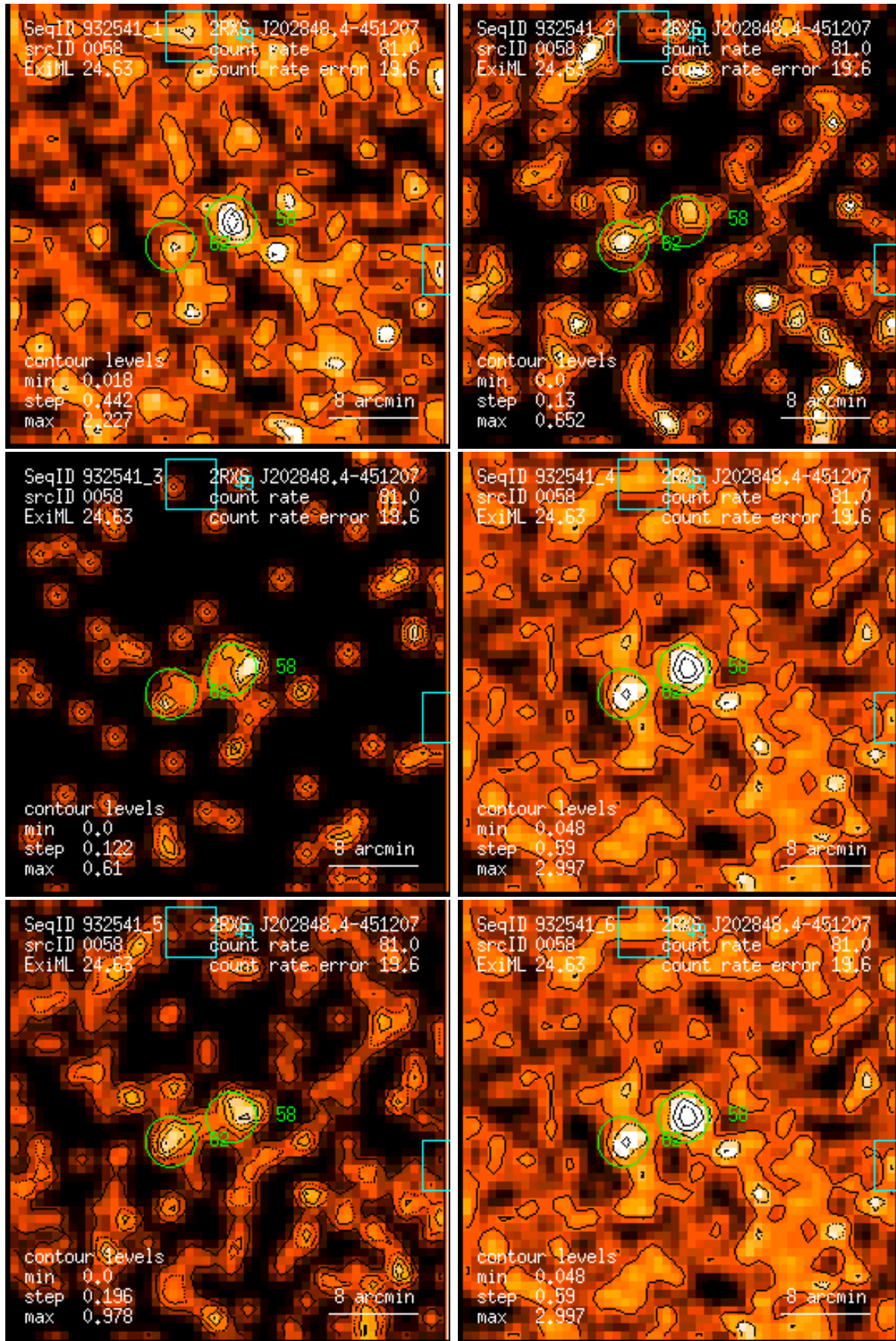
Figure 58: RASS 932541: detection 0058: band rate images, Gaussian filter: (1) PSPC channels 11 – 41, (2) 52 – 90, (3) 91 – 201, (4) 11 – 235, (5) 52 – 201, (6) 11 – 201. Broad band rates in counts/ks. Band rate contour levels in counts/ks/arcmin 2 .
