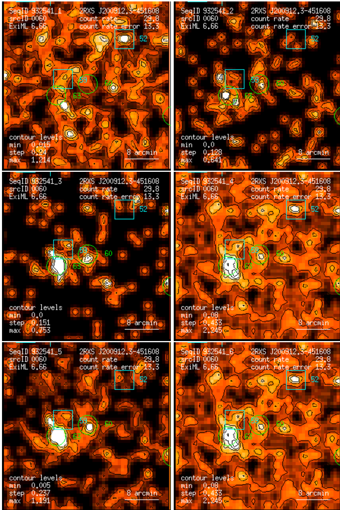
Figure 60: RASS 932541: detection 0060: band rate images, Gaussian filter: (1) PSPC channels 11 – 41, (2) 52 – 90, (3) 91 – 201, (4) 11 – 235, (5) 52 – 201, (6) 11 – 201. Broad band rates in counts/ks. Band rate contour levels in counts/ks/arcmin 2 .
