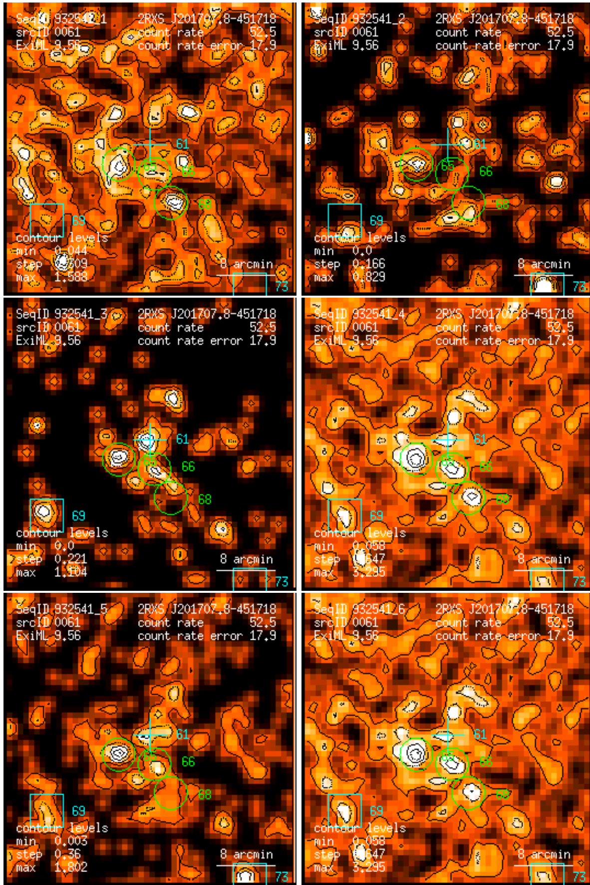
Figure 61: RASS 932541: detection 0061: band rate images, Gaussian filter: (1) PSPC channels 11 – 41, (2) 52 – 90, (3) 91 – 201, (4) 11 – 235, (5) 52 – 201, (6) 11 – 201. Broad band rates in counts/ks. Band rate contour levels in counts/ks/arcmin 2 .
