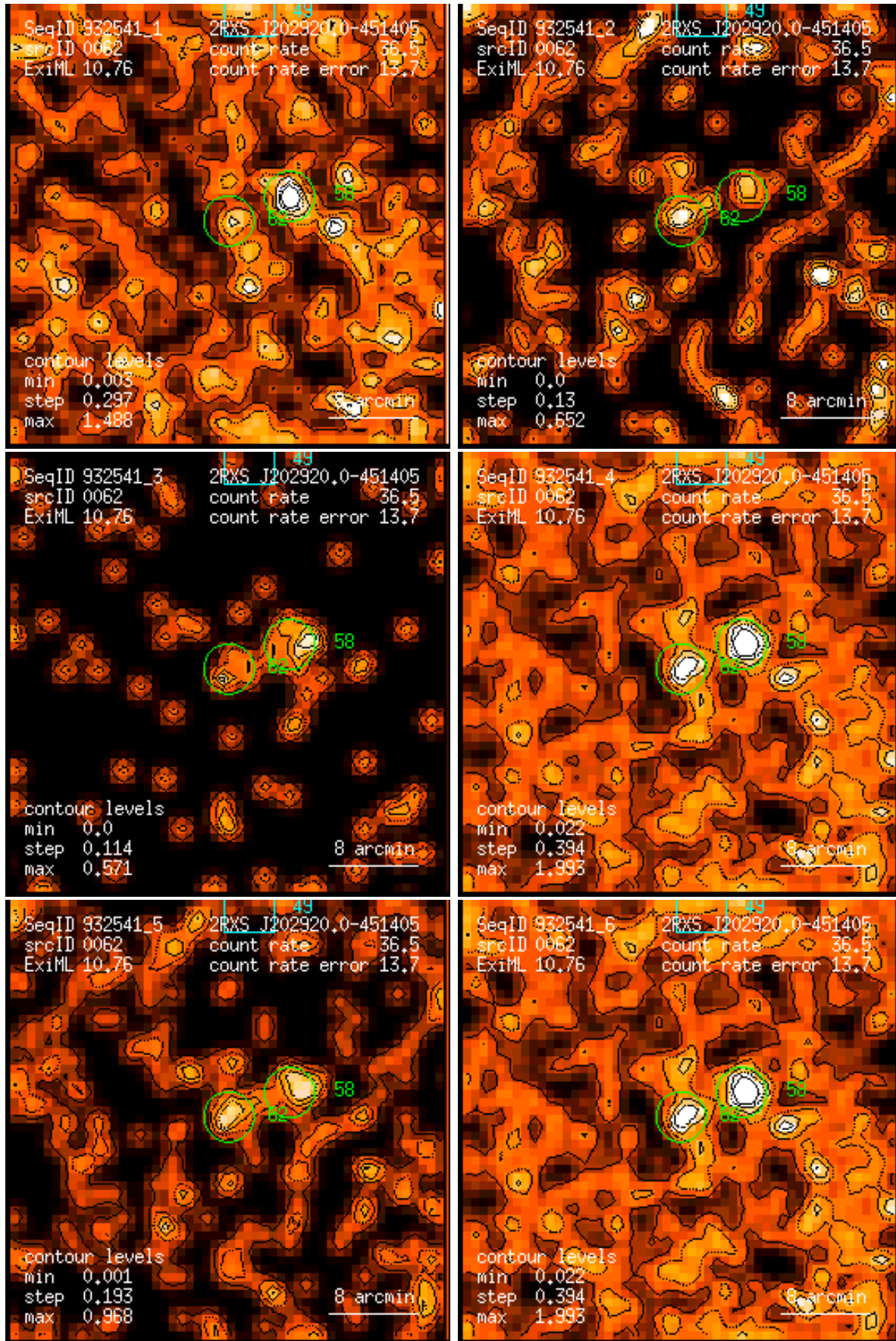
Figure 62: RASS 932541: detection 0062: band rate images, Gaussian filter: (1) PSPC channels 11 – 41, (2) 52 – 90, (3) 91 – 201, (4) 11 – 235, (5) 52 – 201, (6) 11 – 201. Broad band rates in counts/ks. Band rate contour levels in counts/ks/arcmin 2 .
