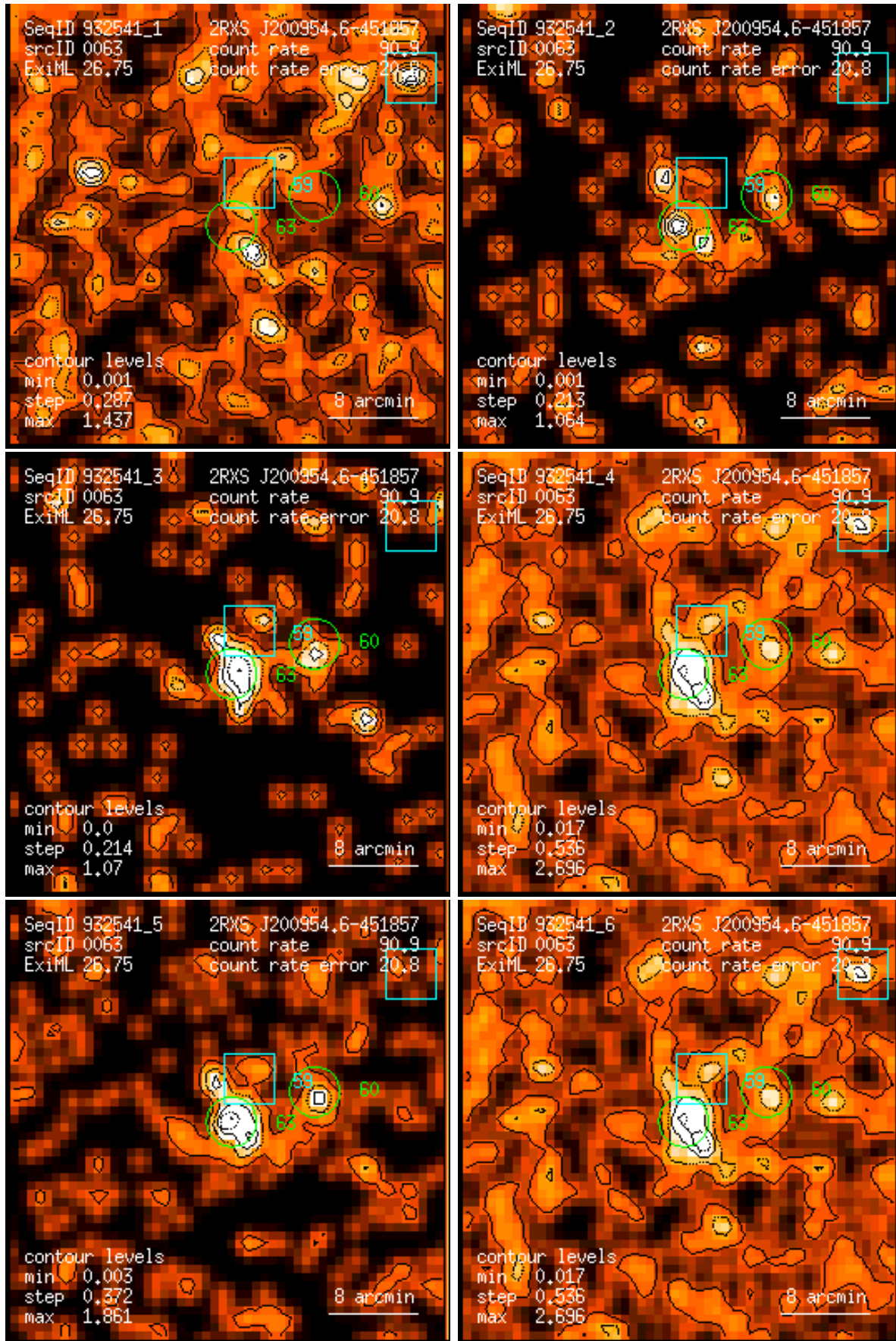
Figure 63: RASS 932541: detection 0063: band rate images, Gaussian filter: (1) PSPC channels 11 – 41, (2) 52 – 90, (3) 91 – 201, (4) 11 – 235, (5) 52 – 201, (6) 11 – 201. Broad band rates in counts/ks. Band rate contour levels in counts/ks/arcmin 2 .
