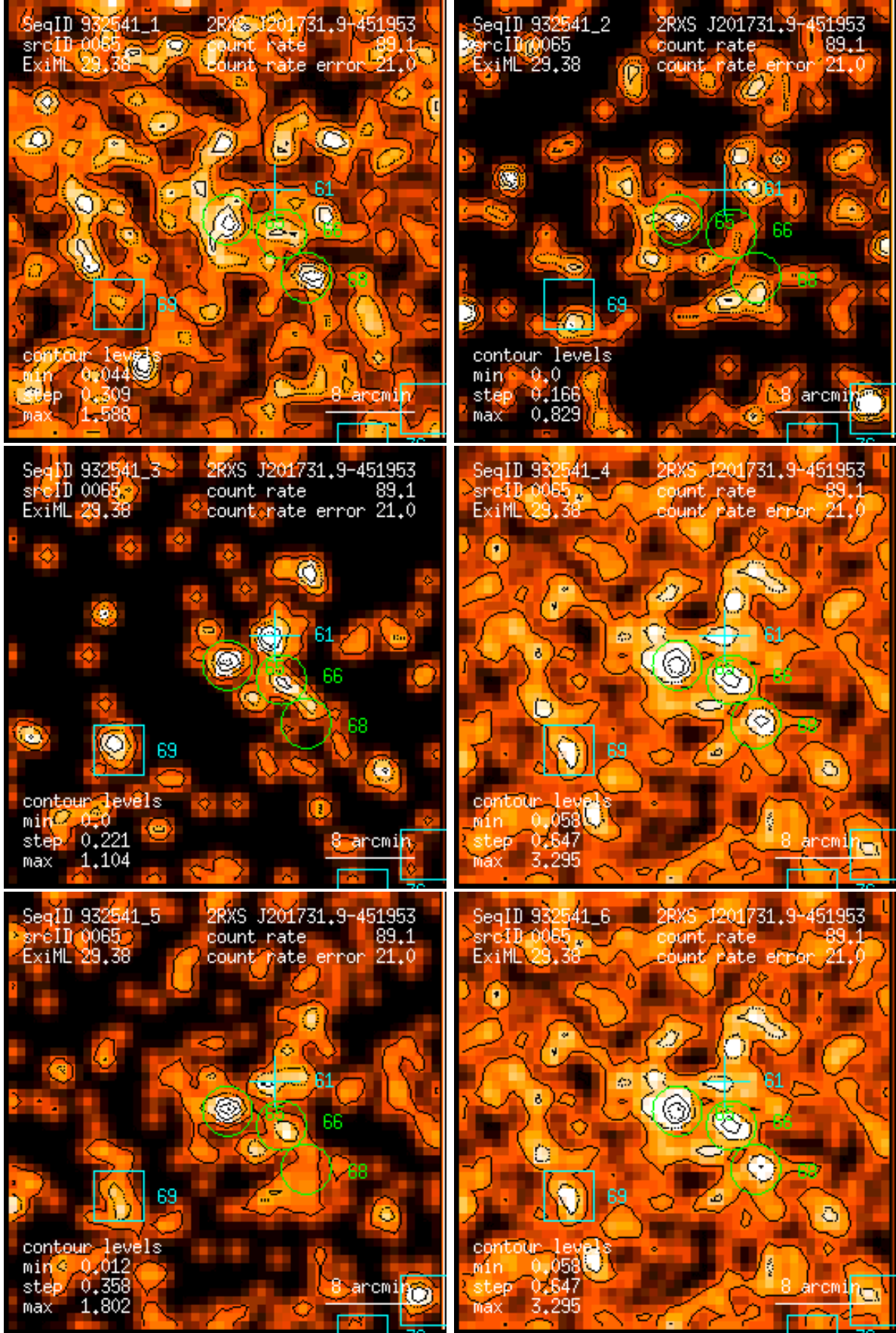
Figure 65: RASS 932541: detection 0065: band rate images, Gaussian filter: (1) PSPC channels 11 – 41, (2) 52 – 90, (3) 91 – 201, (4) 11 – 235, (5) 52 – 201, (6) 11 – 201. Broad band rates in counts/ks. Band rate contour levels in counts/ks/arcmin 2 .
