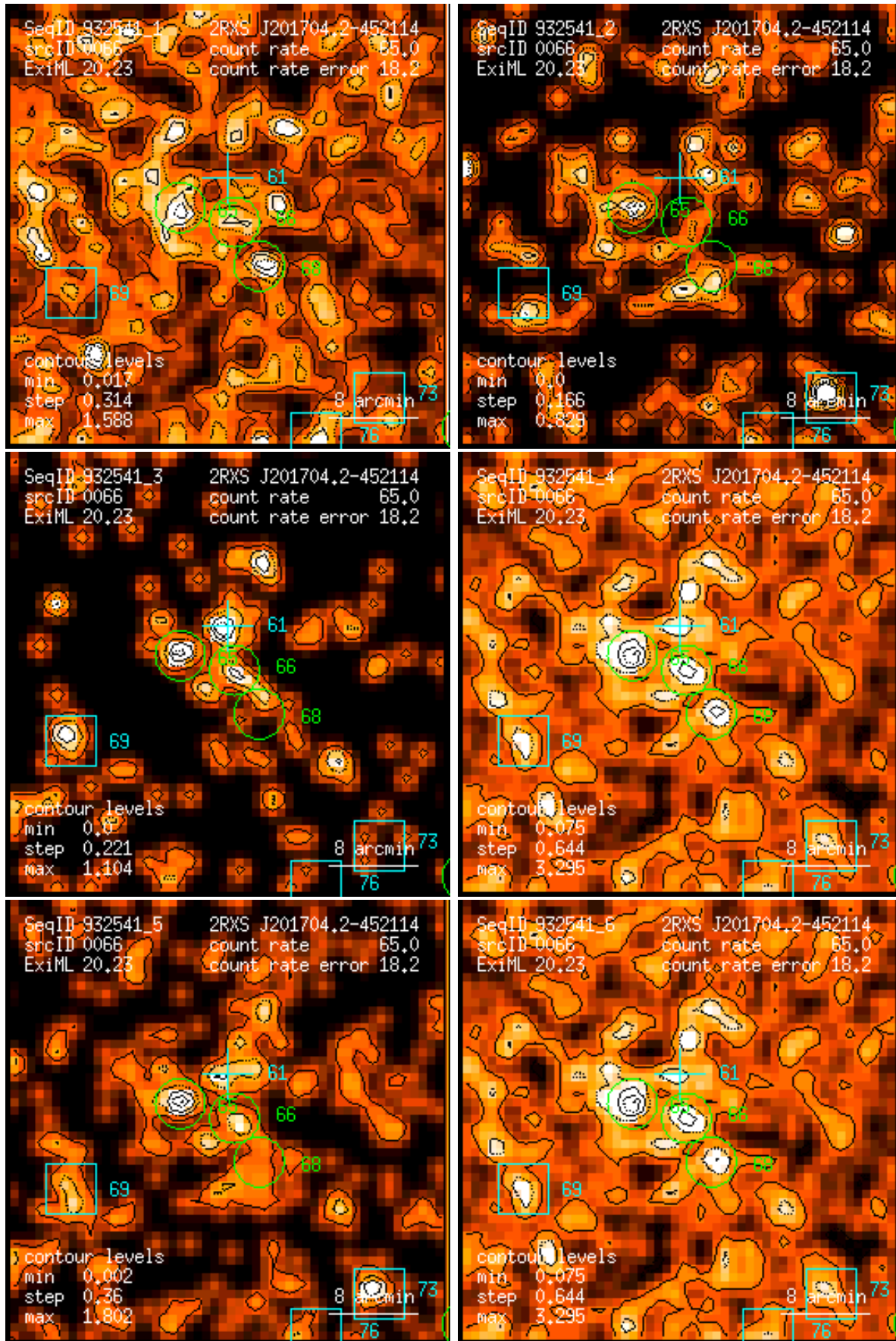
Figure 66: RASS 932541: detection 0066: band rate images, Gaussian filter: (1) PSPC channels 11 – 41, (2) 52 – 90, (3) 91 – 201, (4) 11 – 235, (5) 52 – 201, (6) 11 – 201. Broad band rates in counts/ks. Band rate contour levels in counts/ks/arcmin 2 .
