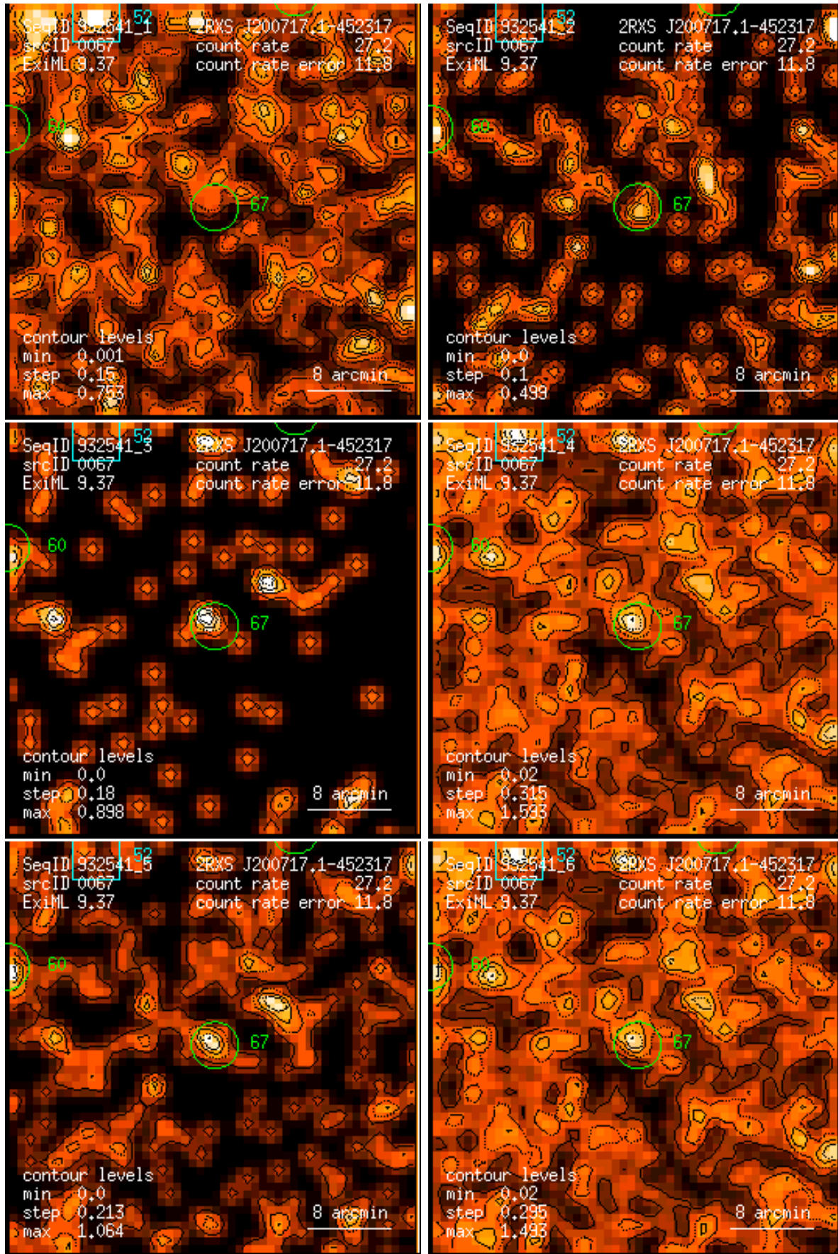
Figure 67: RASS 932541: detection 0067: band rate images, Gaussian filter: (1) PSPC channels 11 – 41, (2) 52 – 90, (3) 91 – 201, (4) 11 – 235, (5) 52 – 201, (6) 11 – 201. Broad band rates in counts/ks. Band rate contour levels in counts/ks/arcmin 2 .
