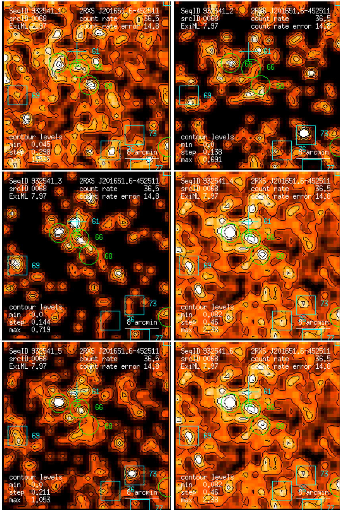
Figure 68: RASS 932541: detection 0068: band rate images, Gaussian filter: (1) PSPC channels 11 – 41, (2) 52 – 90, (3) 91 – 201, (4) 11 – 235, (5) 52 – 201, (6) 11 – 201. Broad band rates in counts/ks. Band rate contour levels in counts/ks/arcmin 2 .
