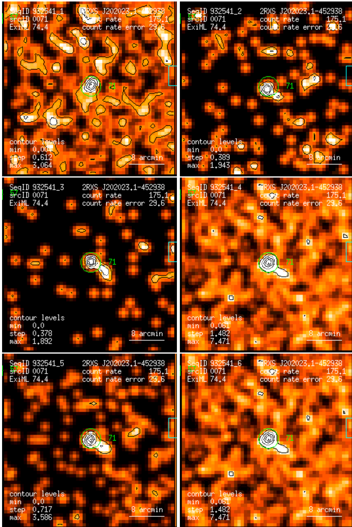
Figure 71: RASS 932541: detection 0071: band rate images, Gaussian filter: (1) PSPC channels 11 – 41, (2) 52 – 90, (3) 91 – 201, (4) 11 – 235, (5) 52 – 201, (6) 11 – 201. Broad band rates in counts/ks. Band rate contour levels in counts/ks/arcmin 2 .
