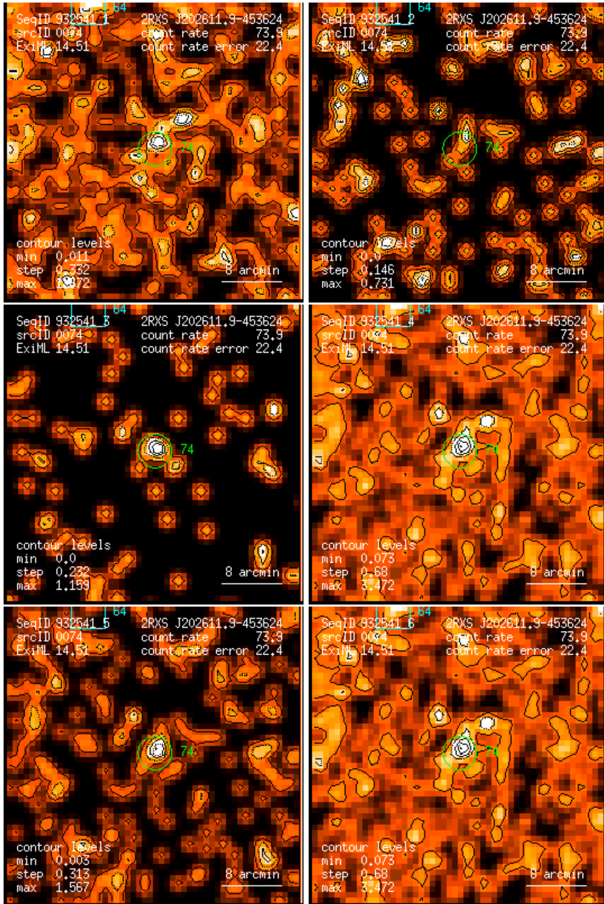
Figure 74: RASS 932541: detection 0074: band rate images, Gaussian filter: (1) PSPC channels 11 – 41, (2) 52 – 90, (3) 91 – 201, (4) 11 – 235, (5) 52 – 201, (6) 11 – 201. Broad band rates in counts/ks. Band rate contour levels in counts/ks/arcmin 2 .
