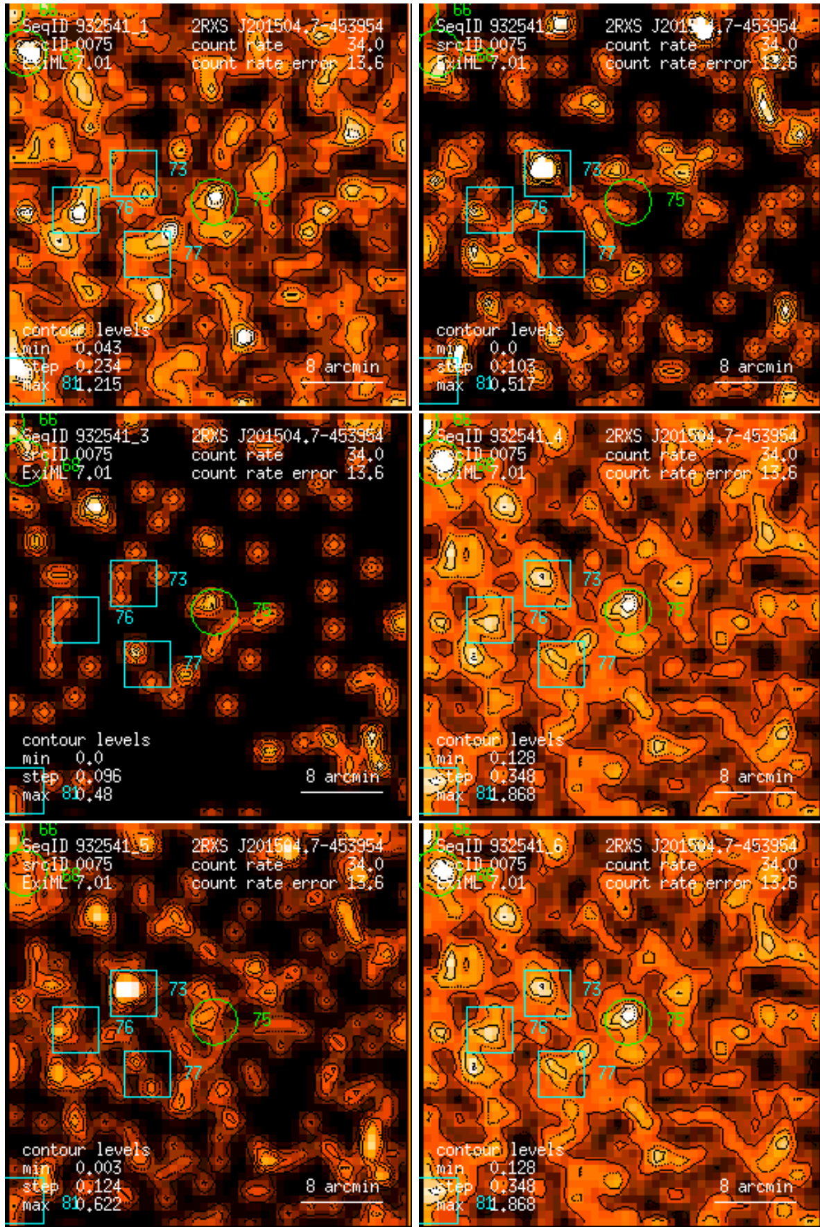
Figure 75: RASS 932541: detection 0075: band rate images, Gaussian filter: (1) PSPC channels 11 – 41, (2) 52 – 90, (3) 91 – 201, (4) 11 – 235, (5) 52 – 201, (6) 11 – 201. Broad band rates in counts/ks. Band rate contour levels in counts/ks/arcmin 2 .
