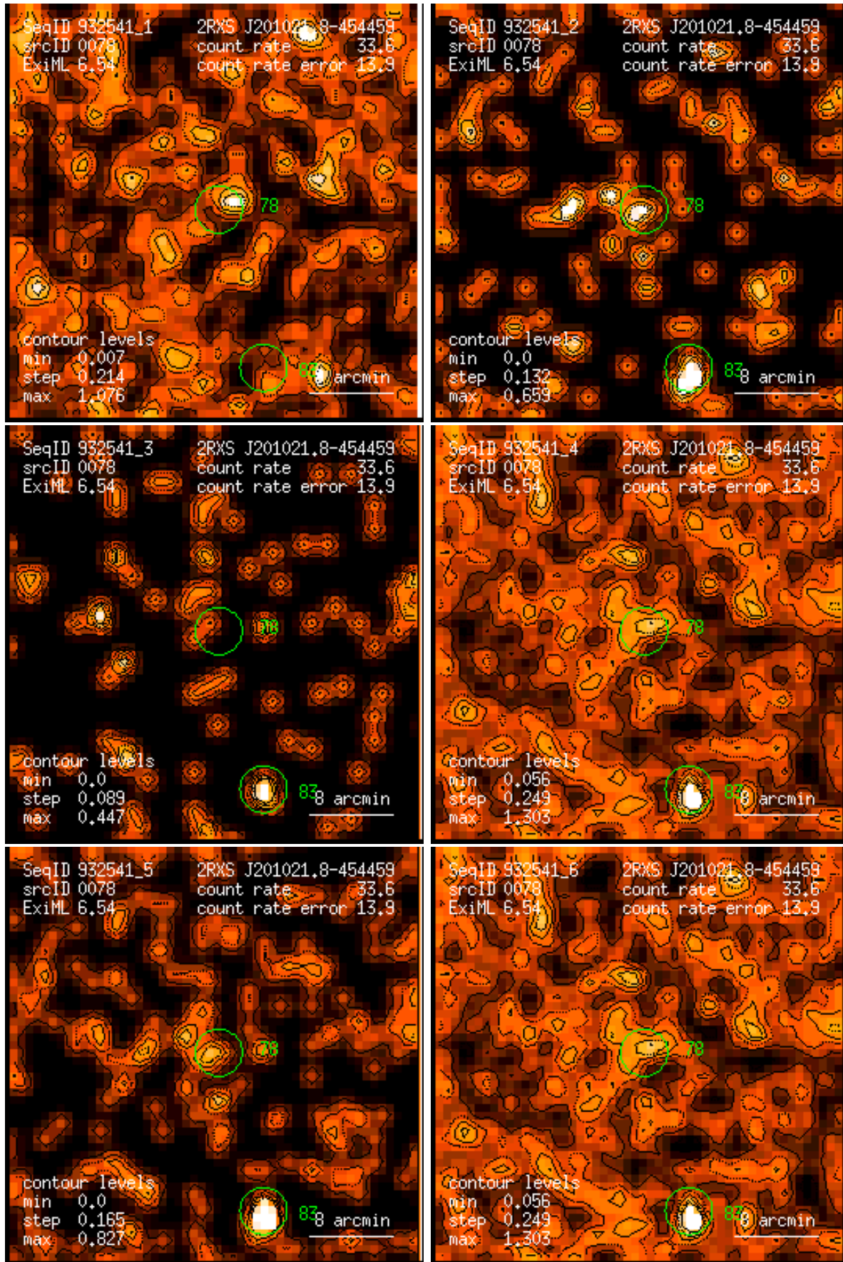
Figure 78: RASS 932541: detection 0078: band rate images, Gaussian filter: (1) PSPC channels 11 – 41, (2) 52 – 90, (3) 91 – 201, (4) 11 – 235, (5) 52 – 201, (6) 11 – 201. Broad band rates in counts/ks. Band rate contour levels in counts/ks/arcmin 2 .
