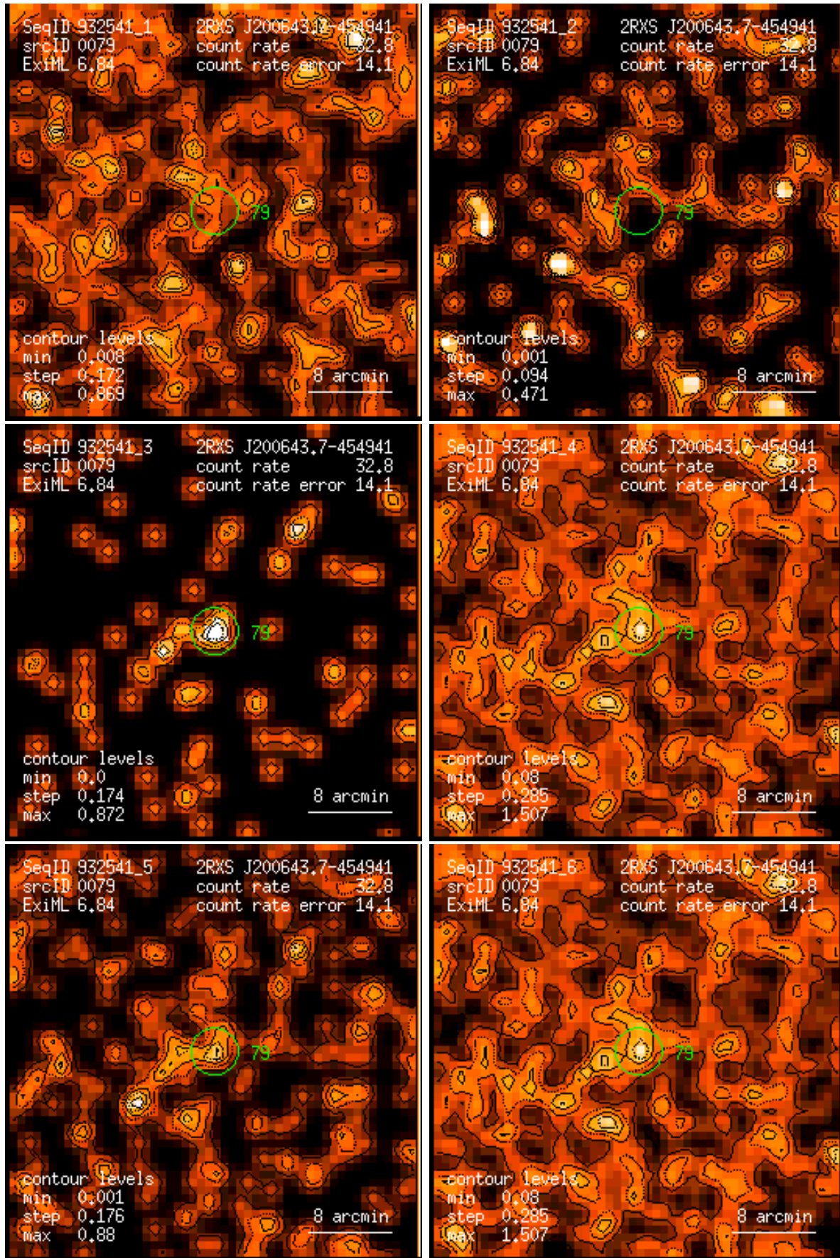
Figure 79: RASS 932541: detection 0079: band rate images, Gaussian filter: (1) PSPC channels 11 – 41, (2) 52 – 90, (3) 91 – 201, (4) 11 – 235, (5) 52 – 201, (6) 11 – 201. Broad band rates in counts/ks. Band rate contour levels in counts/ks/arcmin 2 .
