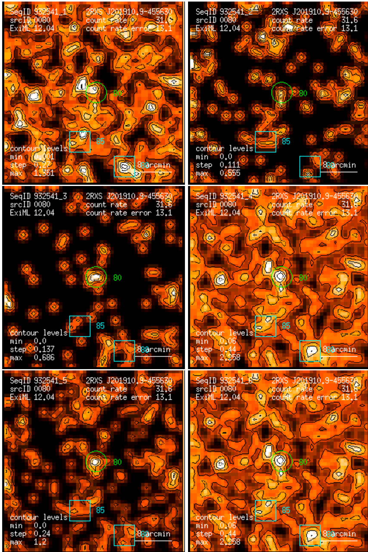
Figure 80: RASS 932541: detection 0080: band rate images, Gaussian filter: (1) PSPC channels 11 – 41, (2) 52 – 90, (3) 91 – 201, (4) 11 – 235, (5) 52 – 201, (6) 11 – 201. Broad band rates in counts/ks. Band rate contour levels in counts/ks/arcmin 2 .
