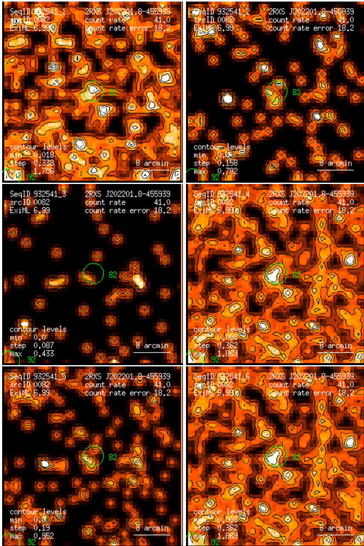
Figure 82: RASS 932541: detection 0082: band rate images, Gaussian filter: (1) PSPC channels 11 – 41, (2) 52 – 90, (3) 91 – 201, (4) 11 – 235, (5) 52 – 201, (6) 11 – 201. Broad band rates in counts/ks. Band rate contour levels in counts/ks/arcmin 2 .
