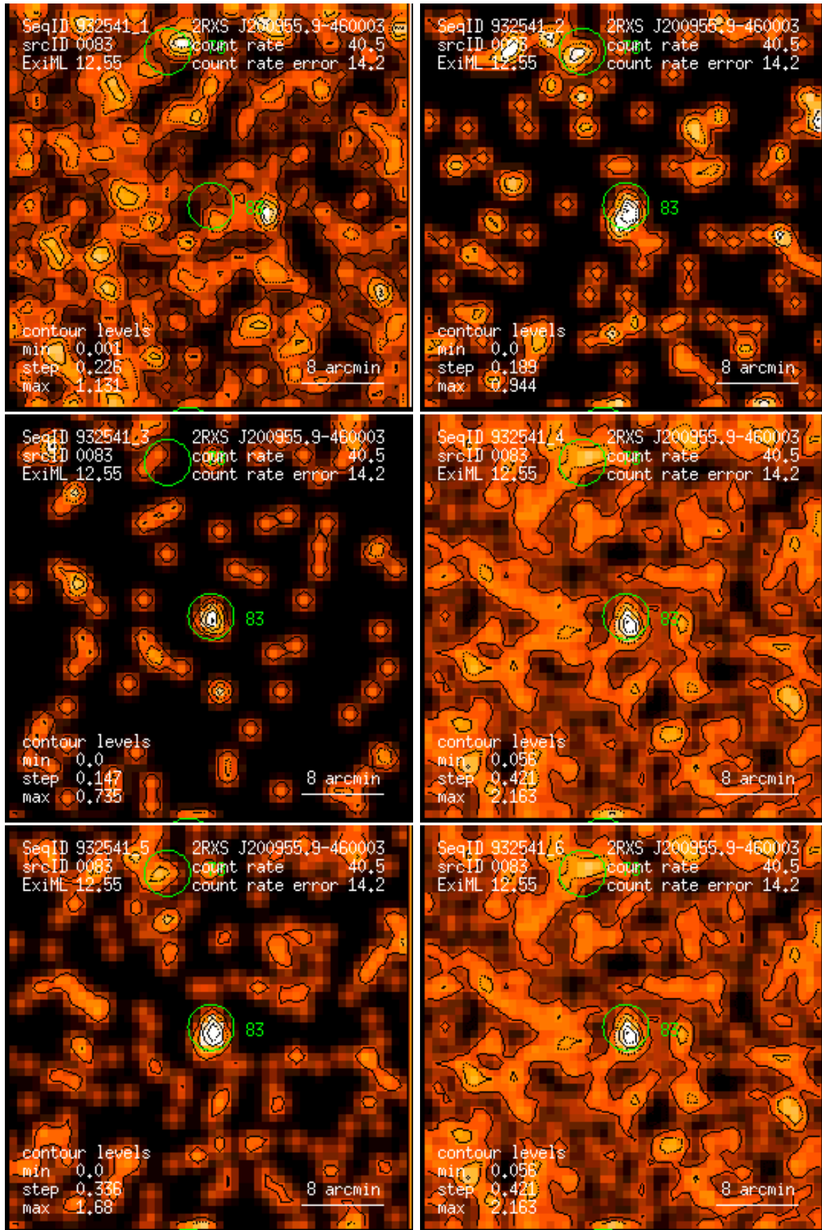
Figure 83: RASS 932541: detection 0083: band rate images, Gaussian filter: (1) PSPC channels 11 – 41, (2) 52 – 90, (3) 91 – 201, (4) 11 – 235, (5) 52 – 201, (6) 11 – 201. Broad band rates in counts/ks. Band rate contour levels in counts/ks/arcmin 2 .
