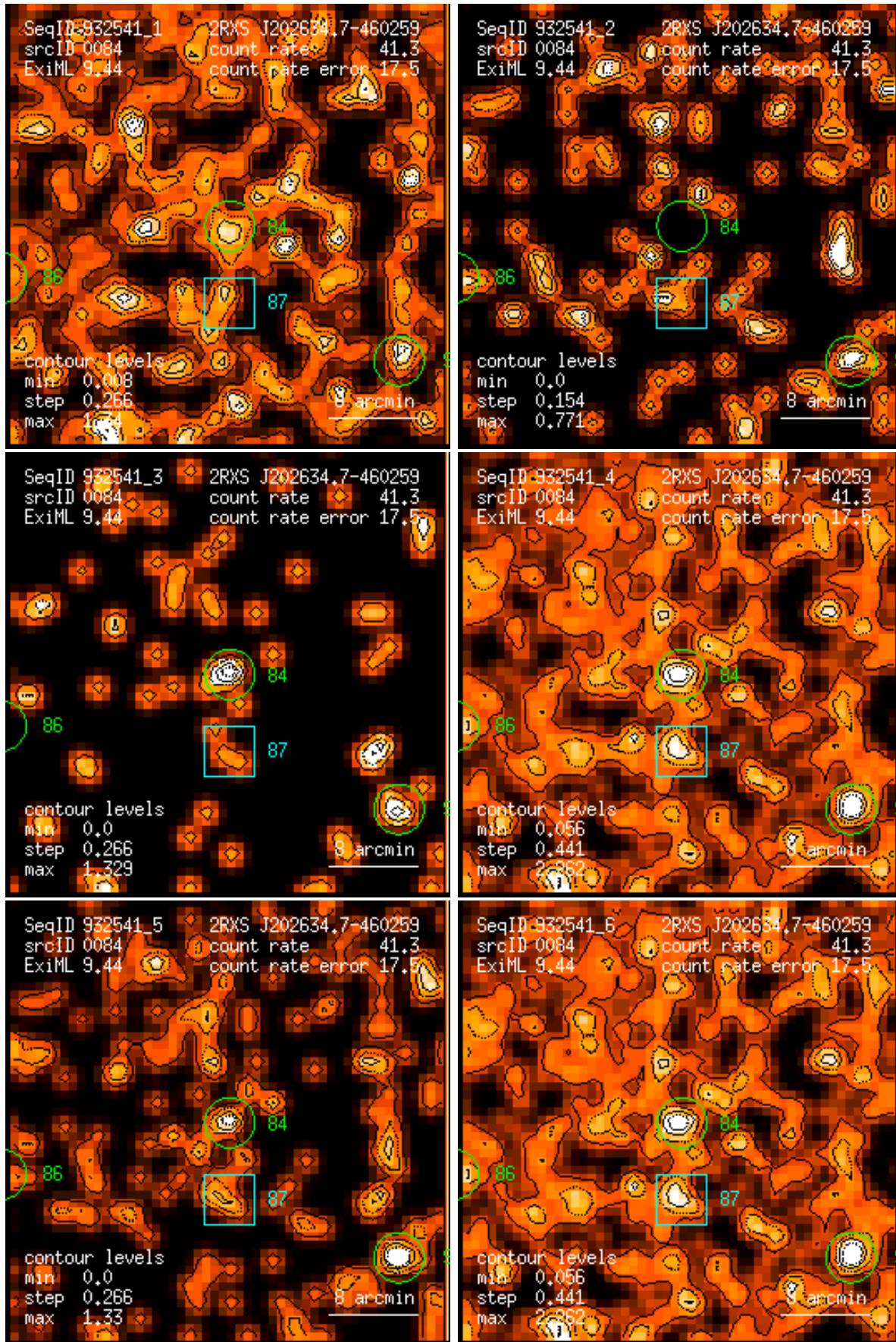
Figure 84: RASS 932541: detection 0084: band rate images, Gaussian filter: (1) PSPC channels 11 – 41, (2) 52 – 90, (3) 91 – 201, (4) 11 – 235, (5) 52 – 201, (6) 11 – 201. Broad band rates in counts/ks. Band rate contour levels in counts/ks/arcmin 2 .
