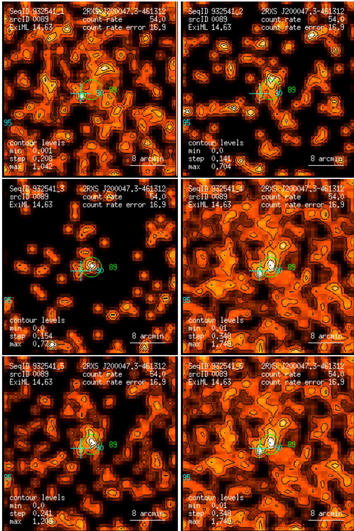
Figure 89: RASS 932541: detection 0089: band rate images, Gaussian filter: (1) PSPC channels 11 – 41, (2) 52 – 90, (3) 91 – 201, (4) 11 – 235, (5) 52 – 201, (6) 11 – 201. Broad band rates in counts/ks. Band rate contour levels in counts/ks/arcmin 2 .
