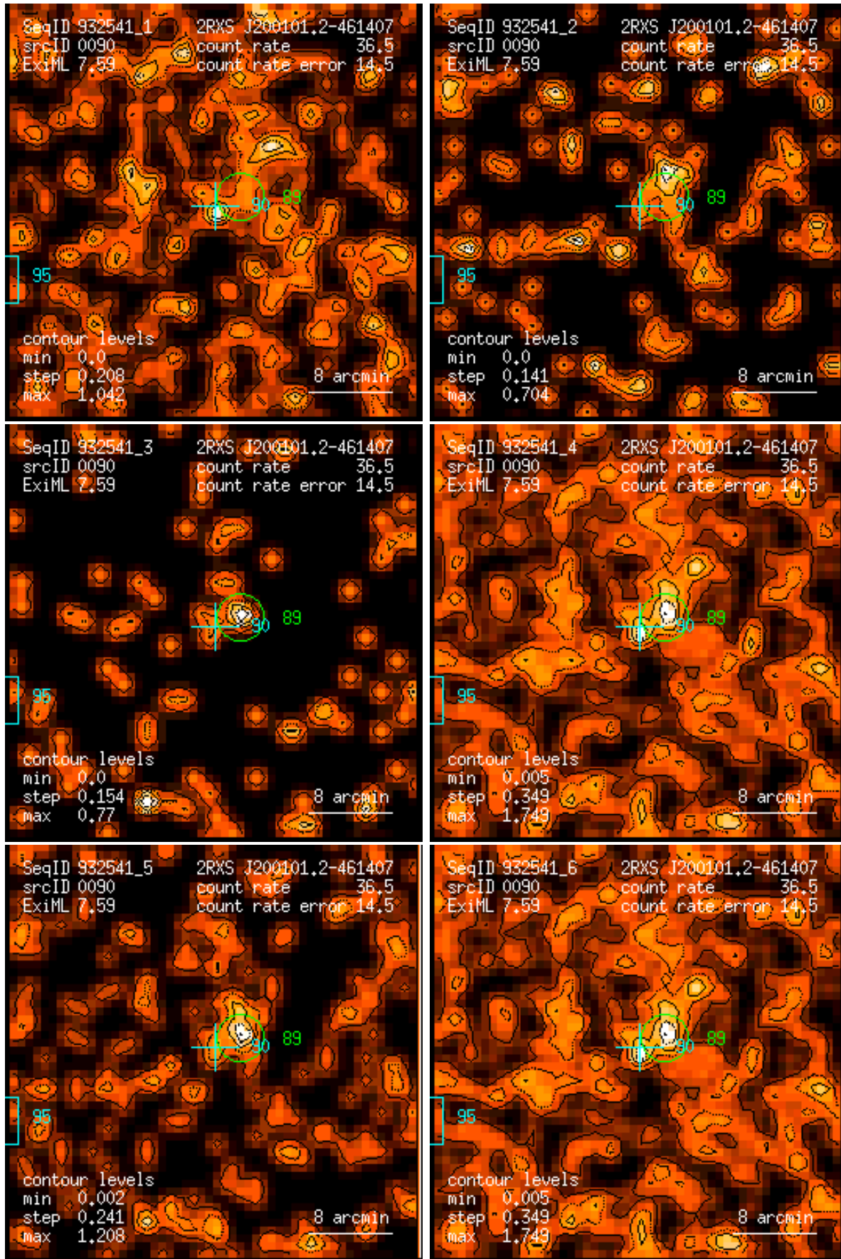
Figure 90: RASS 932541: detection 0090: band rate images, Gaussian filter: (1) PSPC channels 11 – 41, (2) 52 – 90, (3) 91 – 201, (4) 11 – 235, (5) 52 – 201, (6) 11 – 201. Broad band rates in counts/ks. Band rate contour levels in counts/ks/arcmin 2 .
