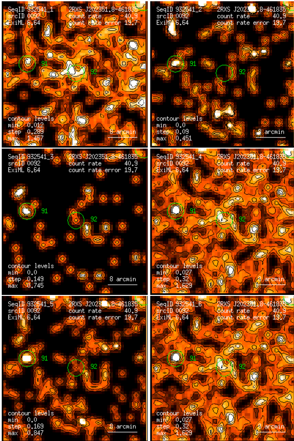
Figure 92: RASS 932541: detection 0092: band rate images, Gaussian filter: (1) PSPC channels 11 – 41, (2) 52 – 90, (3) 91 – 201, (4) 11 – 235, (5) 52 – 201, (6) 11 – 201. Broad band rates in counts/ks. Band rate contour levels in counts/ks/arcmin 2 .
