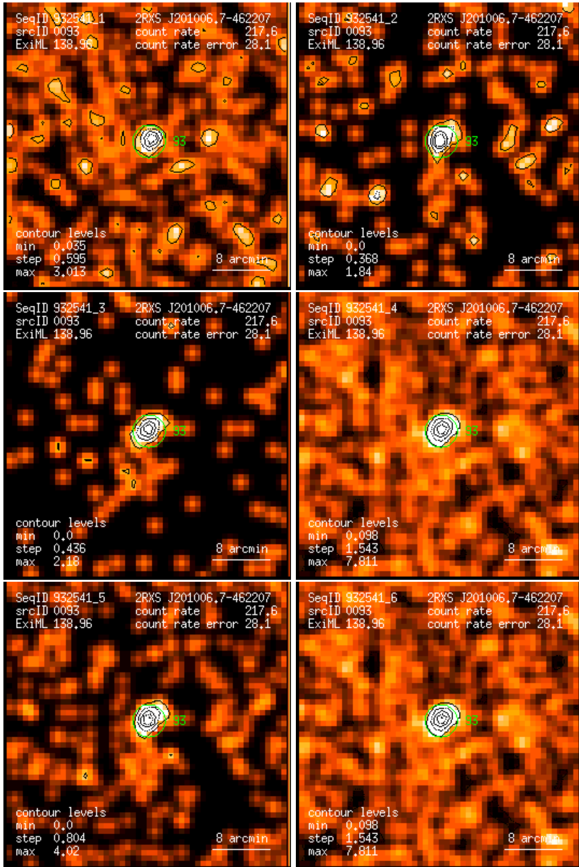
Figure 93: RASS 932541: detection 0093: band rate images, Gaussian filter: (1) PSPC channels 11 – 41, (2) 52 – 90, (3) 91 – 201, (4) 11 – 235, (5) 52 – 201, (6) 11 – 201. Broad band rates in counts/ks. Band rate contour levels in counts/ks/arcmin 2 .
