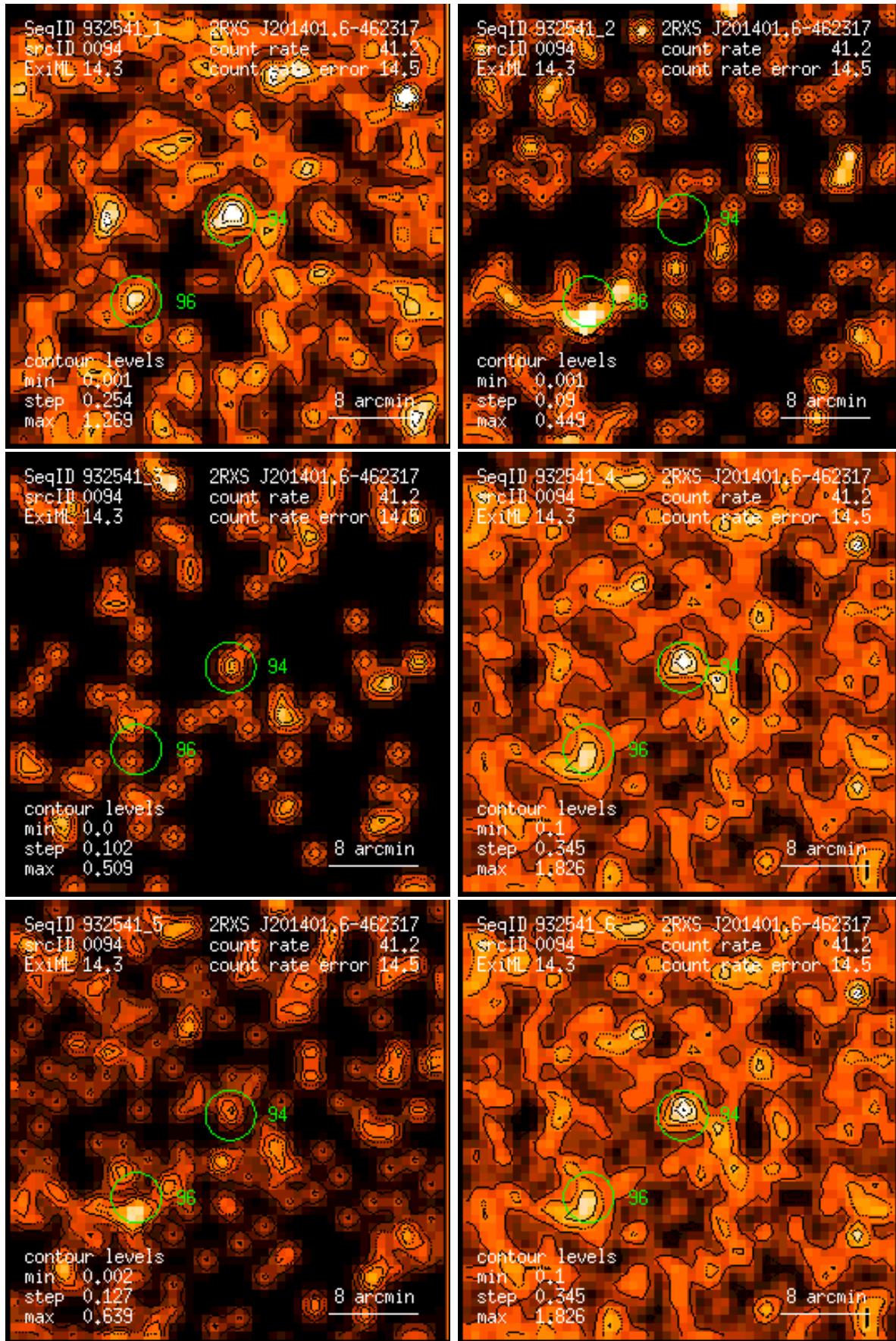
Figure 94: RASS 932541: detection 0094: band rate images, Gaussian filter: (1) PSPC channels 11 – 41, (2) 52 – 90, (3) 91 – 201, (4) 11 – 235, (5) 52 – 201, (6) 11 – 201. Broad band rates in counts/ks. Band rate contour levels in counts/ks/arcmin 2 .
