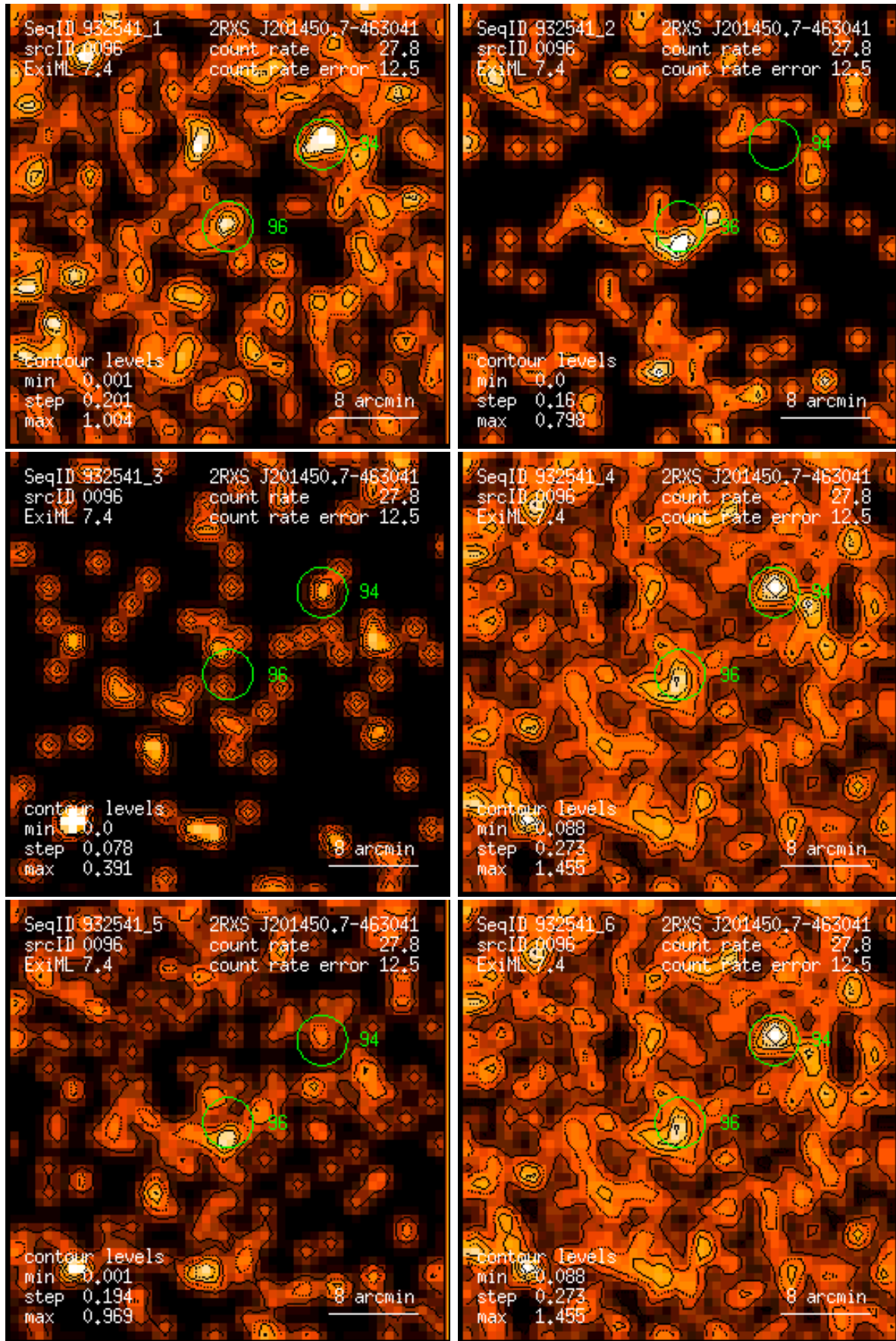
Figure 96: RASS 932541: detection 0096: band rate images, Gaussian filter: (1) PSPC channels 11 – 41, (2) 52 – 90, (3) 91 – 201, (4) 11 – 235, (5) 52 – 201, (6) 11 – 201. Broad band rates in counts/ks. Band rate contour levels in counts/ks/arcmin 2 .
