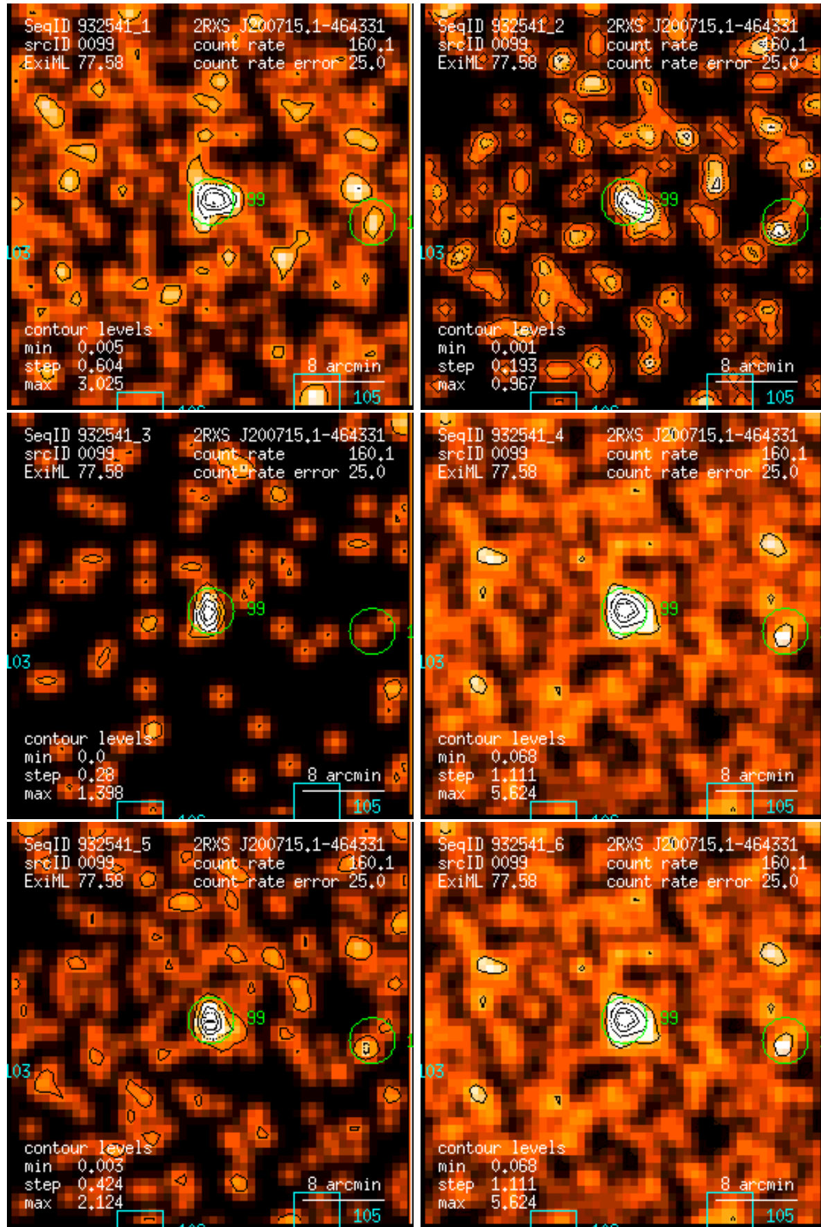
Figure 99: RASS 932541: detection 0099: band rate images, Gaussian filter: (1) PSPC channels 11 – 41, (2) 52 – 90, (3) 91 – 201, (4) 11 – 235, (5) 52 – 201, (6) 11 – 201. Broad band rates in counts/ks. Band rate contour levels in counts/ks/arcmin 2 .
