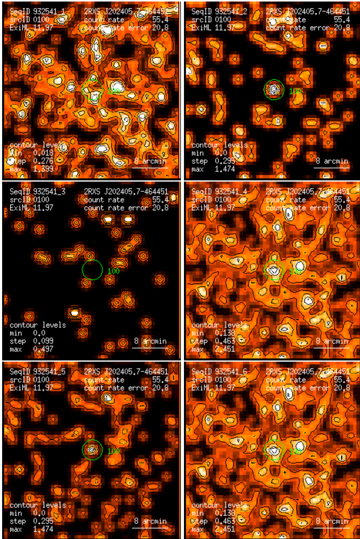
Figure 100: RASS 932541: detection 0100: band rate images, Gaussian filter: (1) PSPC channels 11 – 41, (2) 52 – 90, (3) 91 – 201, (4) 11 – 235, (5) 52 – 201, (6) 11 – 201. Broad band rates in counts/ks. Band rate contour levels in counts/ks/arcmin 2 .
