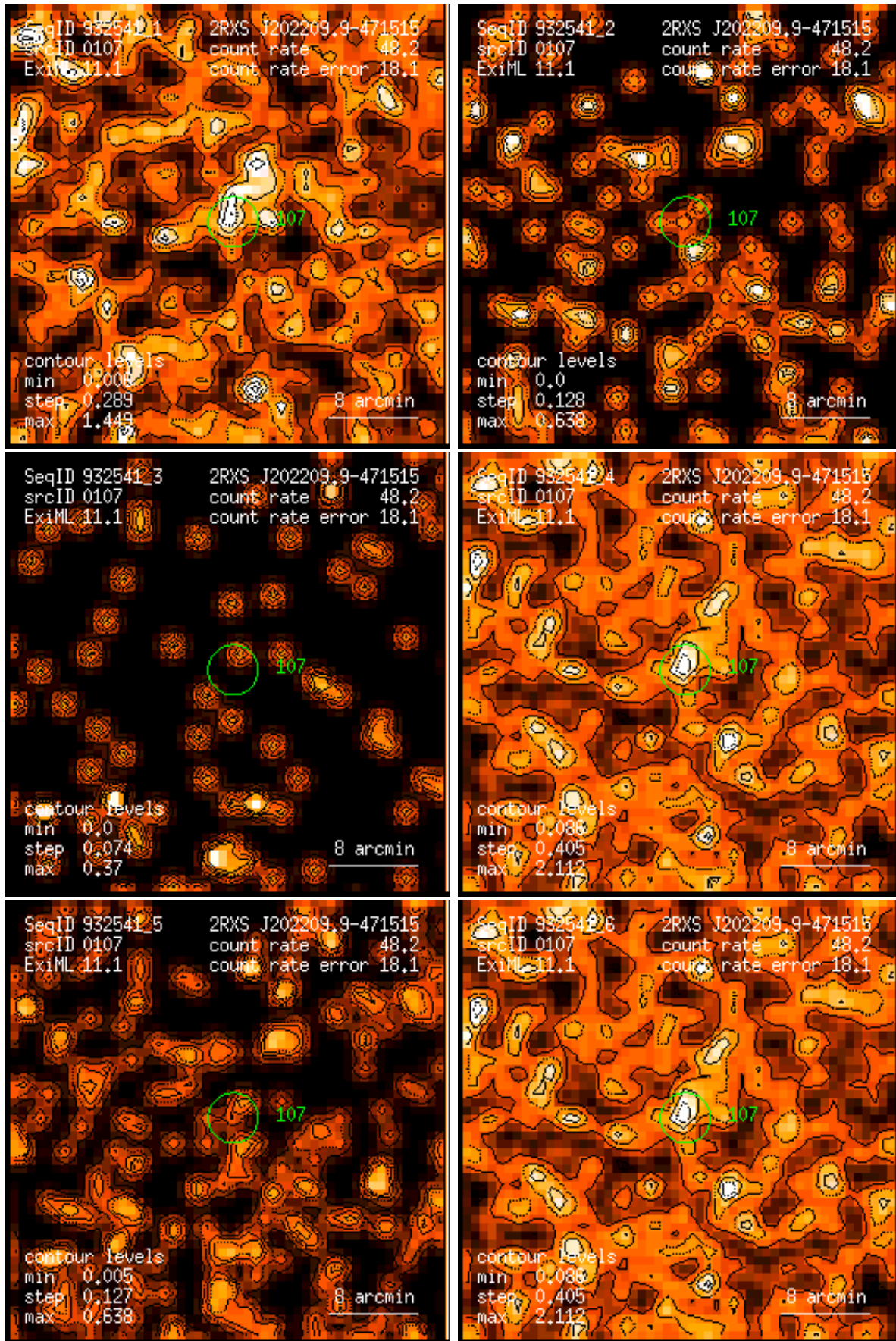
Figure 107: RASS 932541: detection 0107: band rate images, Gaussian filter: (1) PSPC channels 11 – 41, (2) 52 – 90, (3) 91 – 201, (4) 11 – 235, (5) 52 – 201, (6) 11 – 201. Broad band rates in counts/ks. Band rate contour levels in counts/ks/arcmin 2 .
