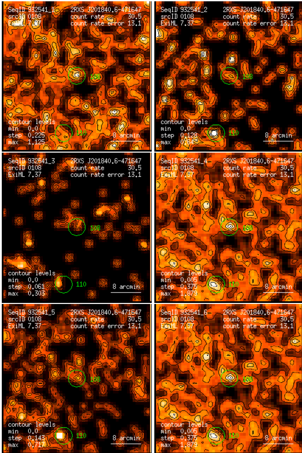
Figure 108: RASS 932541: detection 0108: band rate images, Gaussian filter: (1) PSPC channels 11 – 41, (2) 52 – 90, (3) 91 – 201, (4) 11 – 235, (5) 52 – 201, (6) 11 – 201. Broad band rates in counts/ks. Band rate contour levels in counts/ks/arcmin 2 .
