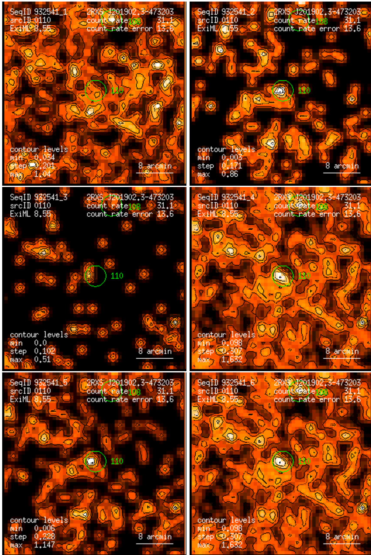
Figure 110: RASS 932541: detection 0110: band rate images, Gaussian filter: (1) PSPC channels 11 – 41, (2) 52 – 90, (3) 91 – 201, (4) 11 – 235, (5) 52 – 201, (6) 11 – 201. Broad band rates in counts/ks. Band rate contour levels in counts/ks/arcmin 2 .
