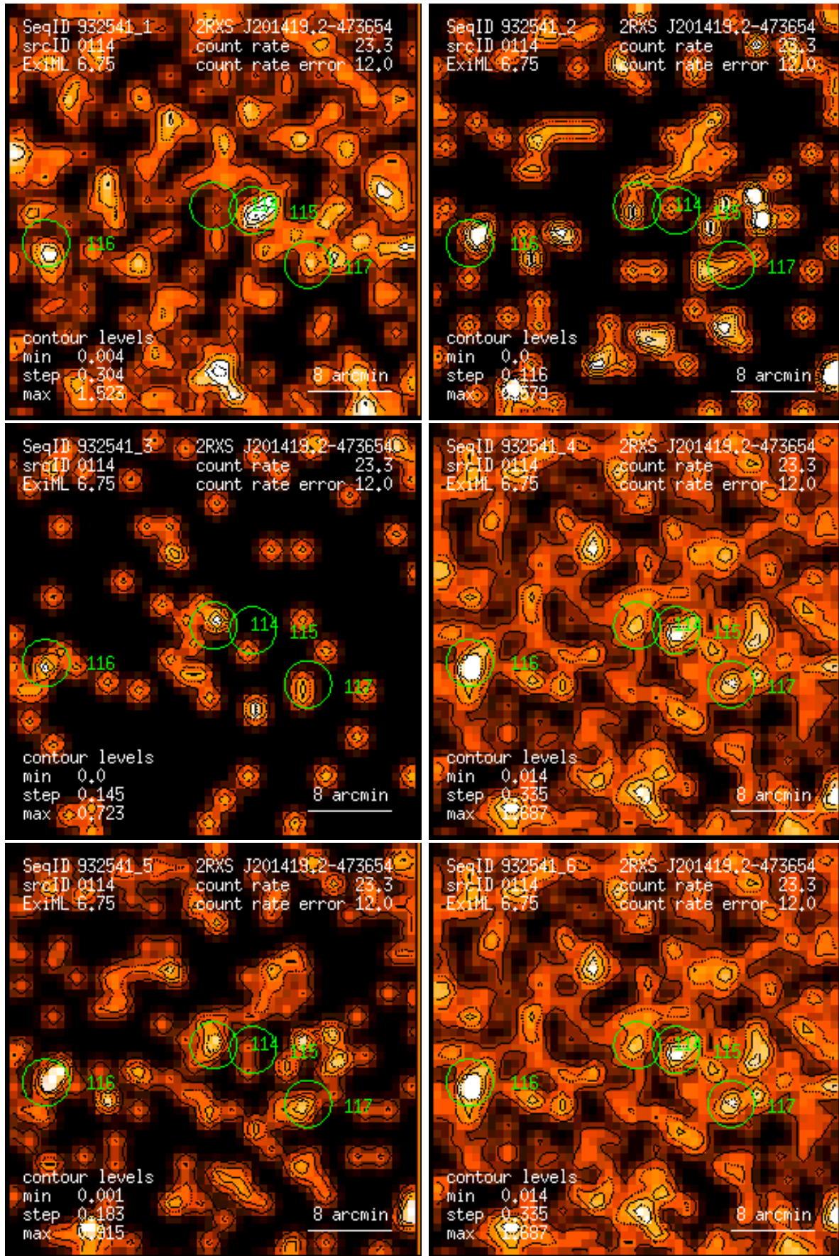
Figure 114: RASS 932541: detection 0114: band rate images, Gaussian filter: (1) PSPC channels 11 – 41, (2) 52 – 90, (3) 91 – 201, (4) 11 – 235, (5) 52 – 201, (6) 11 – 201. Broad band rates in counts/ks. Band rate contour levels in counts/ks/arcmin 2 .
