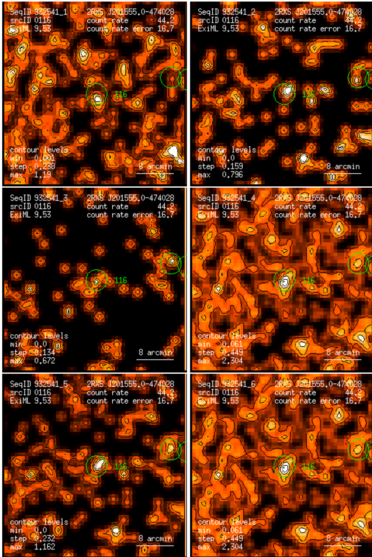
Figure 116: RASS 932541: detection 0116: band rate images, Gaussian filter: (1) PSPC channels 11 – 41, (2) 52 – 90, (3) 91 – 201, (4) 11 – 235, (5) 52 – 201, (6) 11 – 201. Broad band rates in counts/ks. Band rate contour levels in counts/ks/arcmin 2 .
