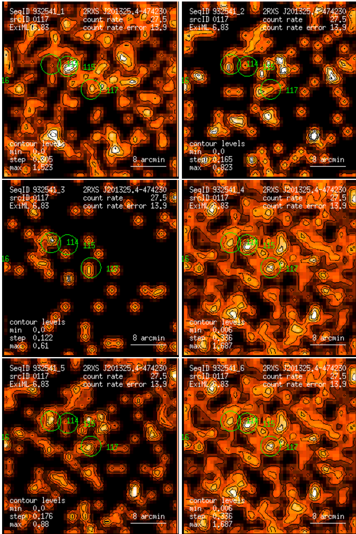
Figure 117: RASS 932541: detection 0117: band rate images, Gaussian filter: (1) PSPC channels 11 – 41, (2) 52 – 90, (3) 91 – 201, (4) 11 – 235, (5) 52 – 201, (6) 11 – 201. Broad band rates in counts/ks. Band rate contour levels in counts/ks/arcmin 2 .
