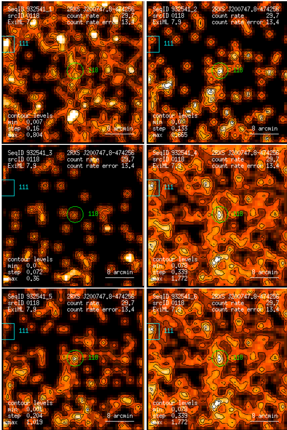
Figure 118: RASS 932541: detection 0118: band rate images, Gaussian filter: (1) PSPC channels 11 – 41, (2) 52 – 90, (3) 91 – 201, (4) 11 – 235, (5) 52 – 201, (6) 11 – 201. Broad band rates in counts/ks. Band rate contour levels in counts/ks/arcmin 2 .
