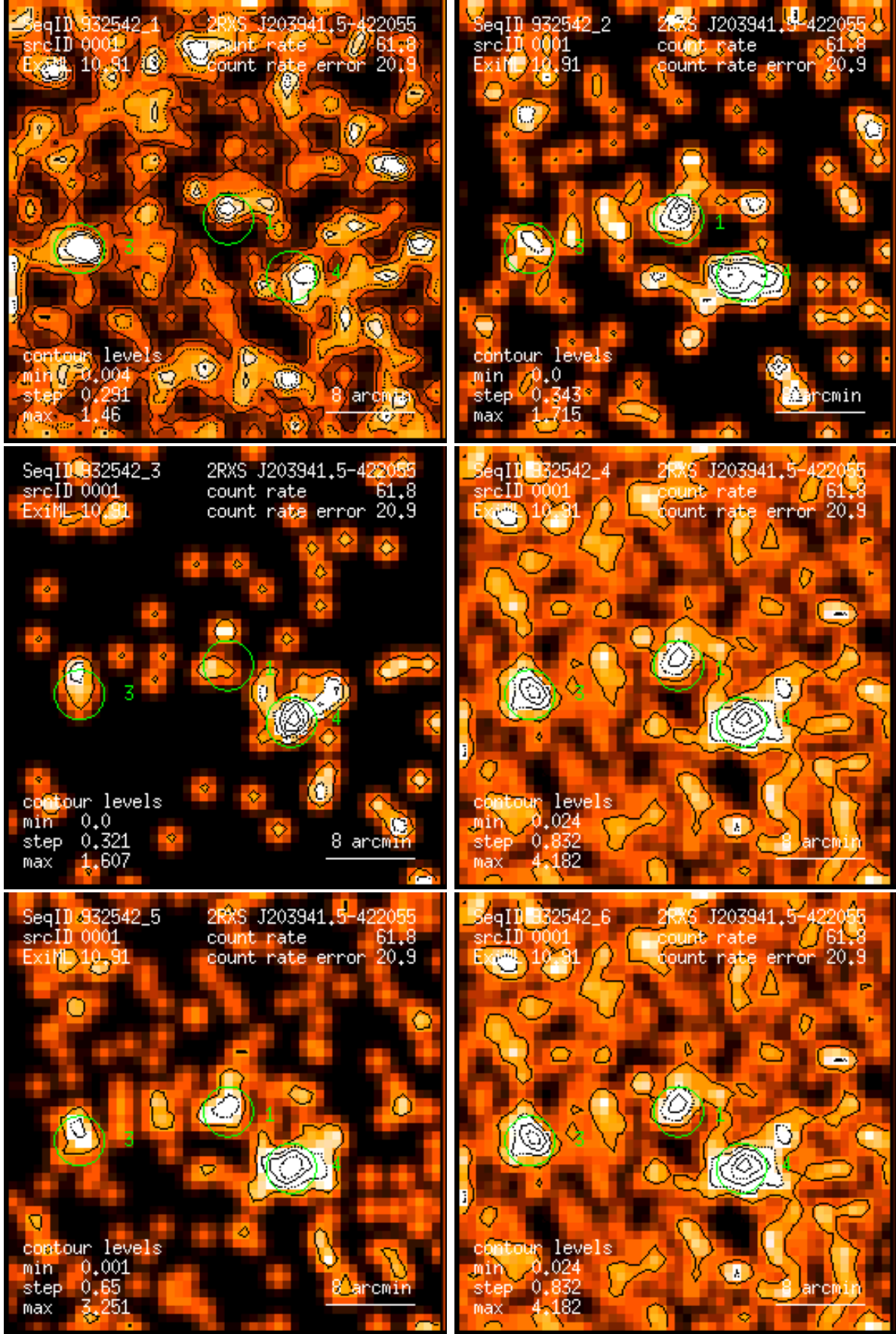
Figure 1: RASS 932542: detection 0001: band rate images, Gaussian filter: (1) PSPC channels 11 – 41, (2) 52 – 90, (3) 91 – 201, (4) 11 – 235, (5) 52 – 201, (6) 11 – 201. Broad band rates in counts/ks. Band rate contour levels in counts/ks/arcmin 2 .
