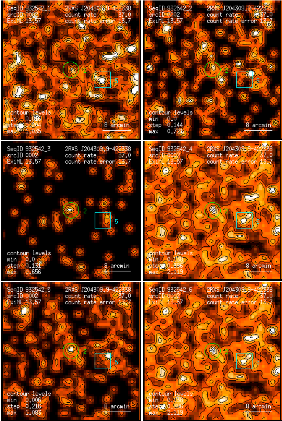
Figure 2: RASS 932542: detection 0002: band rate images, Gaussian filter: (1) PSPC channels 11 – 41, (2) 52 – 90, (3) 91 – 201, (4) 11 – 235, (5) 52 – 201, (6) 11 – 201. Broad band rates in counts/ks. Band rate contour levels in counts/ks/arcmin 2 .
