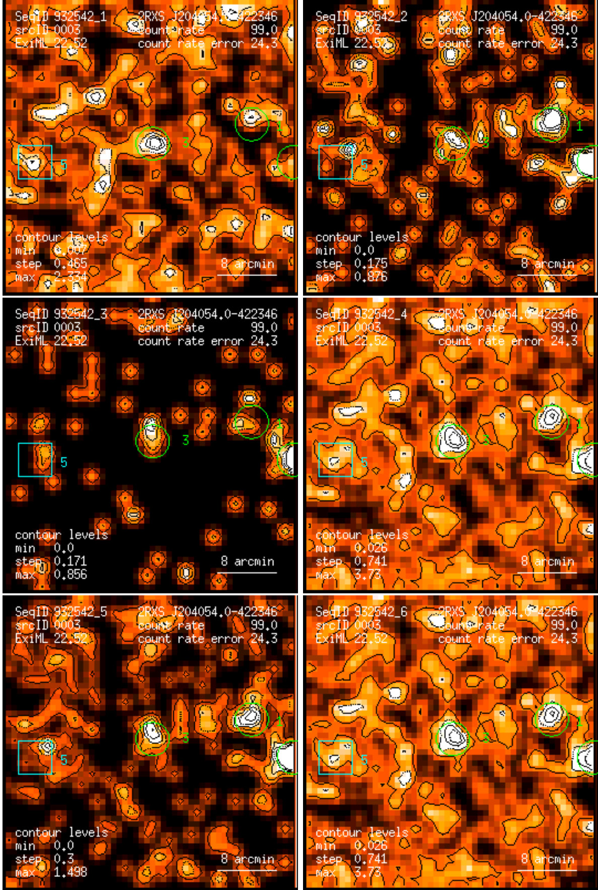
Figure 3: RASS 932542: detection 0003: band rate images, Gaussian filter: (1) PSPC channels 11 – 41, (2) 52 – 90, (3) 91 – 201, (4) 11 – 235, (5) 52 – 201, (6) 11 – 201. Broad band rates in counts/ks. Band rate contour levels in counts/ks/arcmin 2 .
