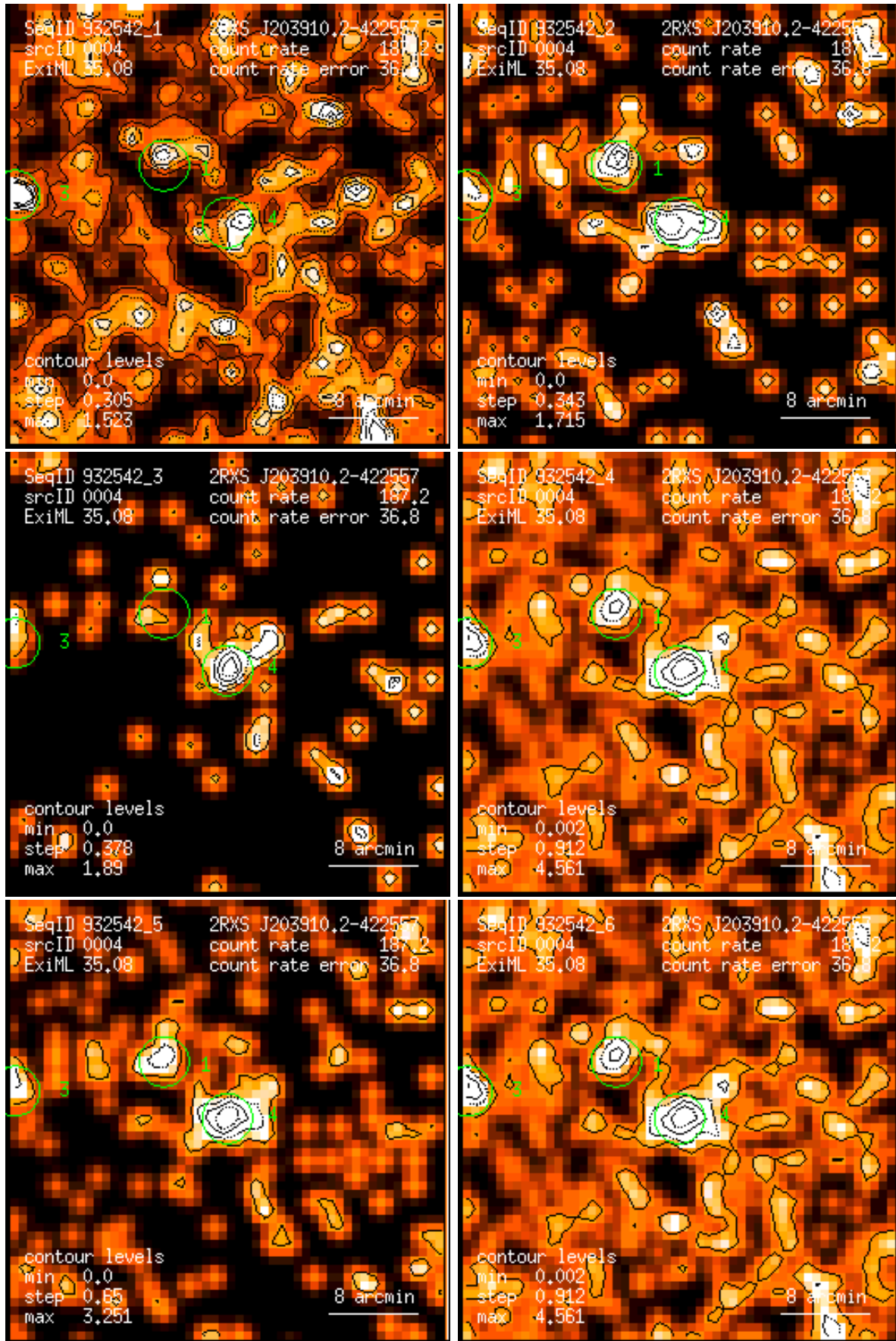
Figure 4: RASS 932542: detection 0004: band rate images, Gaussian filter: (1) PSPC channels 11 – 41, (2) 52 – 90, (3) 91 – 201, (4) 11 – 235, (5) 52 – 201, (6) 11 – 201. Broad band rates in counts/ks. Band rate contour levels in counts/ks/arcmin 2 .
