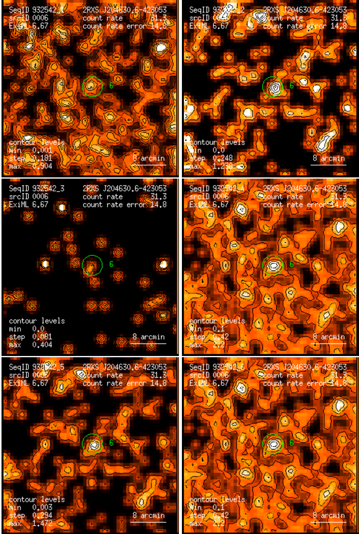
Figure 6: RASS 932542: detection 0006: band rate images, Gaussian filter: (1) PSPC channels 11 – 41, (2) 52 – 90, (3) 91 – 201, (4) 11 – 235, (5) 52 – 201, (6) 11 – 201. Broad band rates in counts/ks. Band rate contour levels in counts/ks/arcmin 2 .
