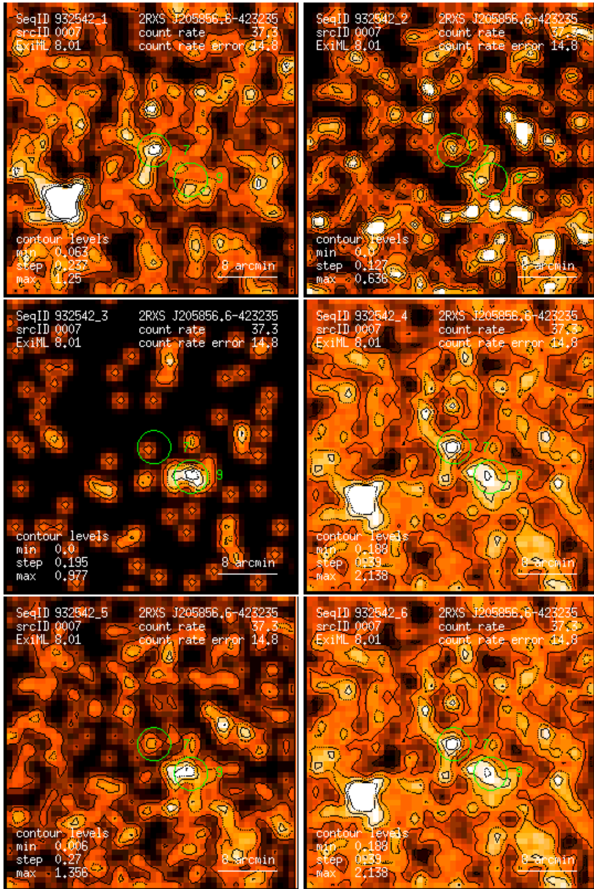
Figure 7: RASS 932542: detection 0007: band rate images, Gaussian filter: (1) PSPC channels 11 – 41, (2) 52 – 90, (3) 91 – 201, (4) 11 – 235, (5) 52 – 201, (6) 11 – 201. Broad band rates in counts/ks. Band rate contour levels in counts/ks/arcmin 2 .
