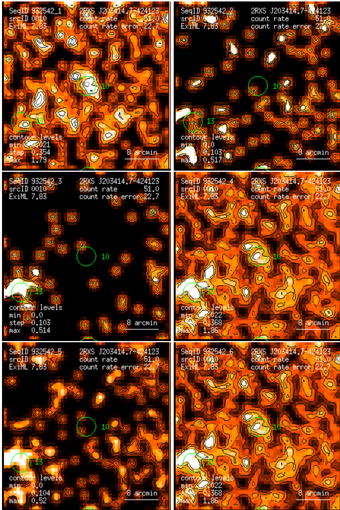
Figure 10: RASS 932542: detection 0010: band rate images, Gaussian filter: (1) PSPC channels 11 – 41, (2) 52 – 90, (3) 91 – 201, (4) 11 – 235, (5) 52 – 201, (6) 11 – 201. Broad band rates in counts/ks. Band rate contour levels in counts/ks/arcmin 2 .
